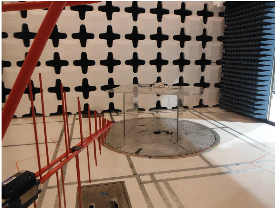
Figure 1: Radiated Emission 30MHz-1Ghz set up
