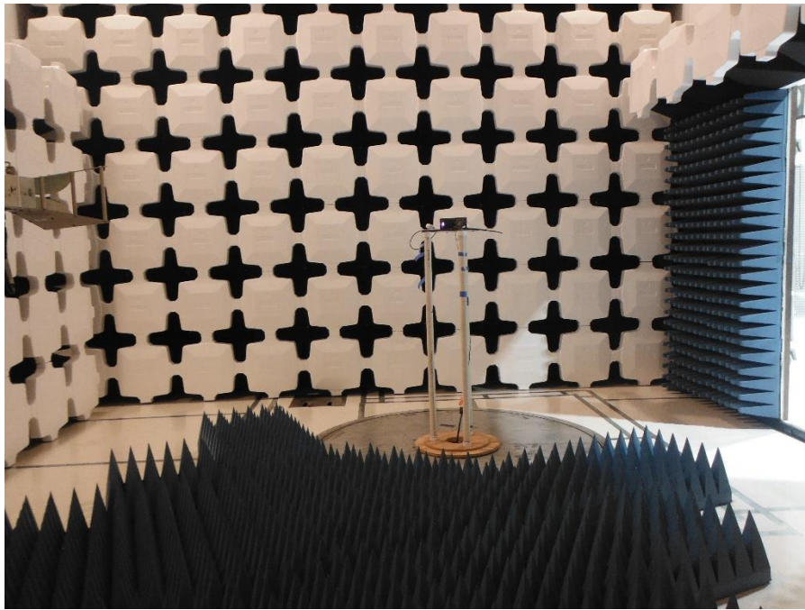
Figure 3: Radiated Emission 1GHz-18GHz set up
