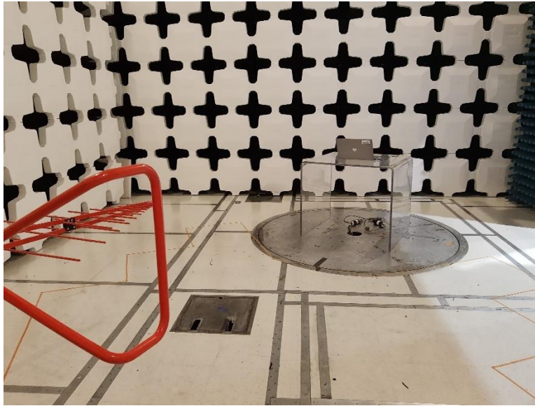
Photograph 1. Radiated Cabinet Spurious Emissions Test Setup, 30-1000MHz
