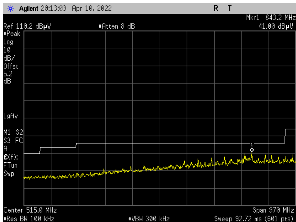
Figure 21. Zigbee_High Ch_2475MHz_2MBit_15.209_30-1000MHz_Peak_Port 1
