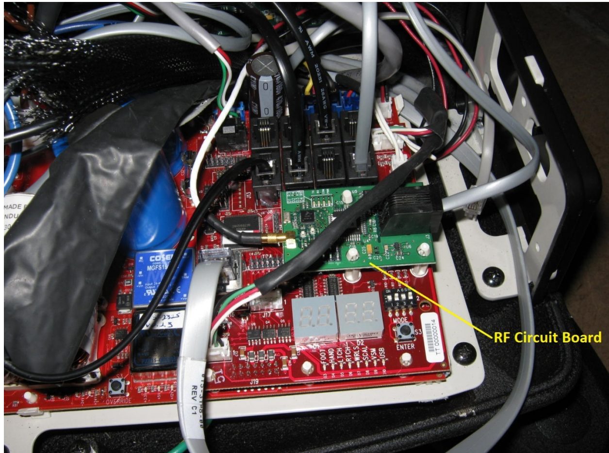
RF Circuit Board installed in chair base
