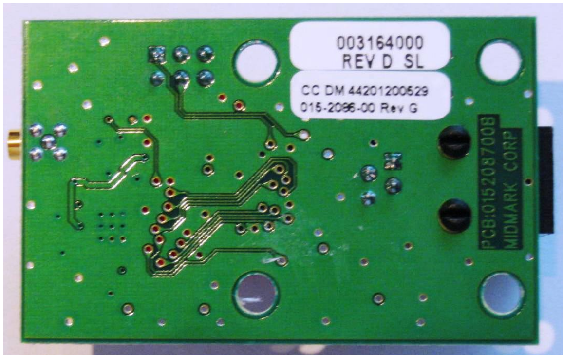
Circuit Board - Side 2
