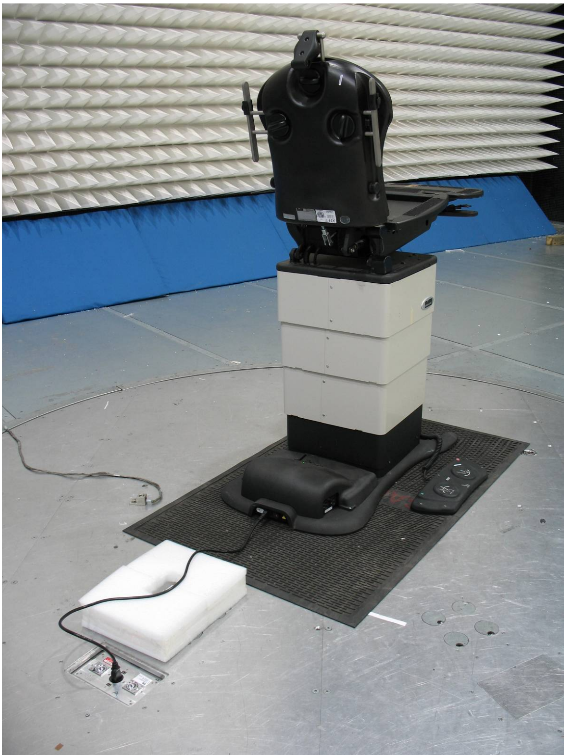
Conducted Emissions on the AC Power Input
