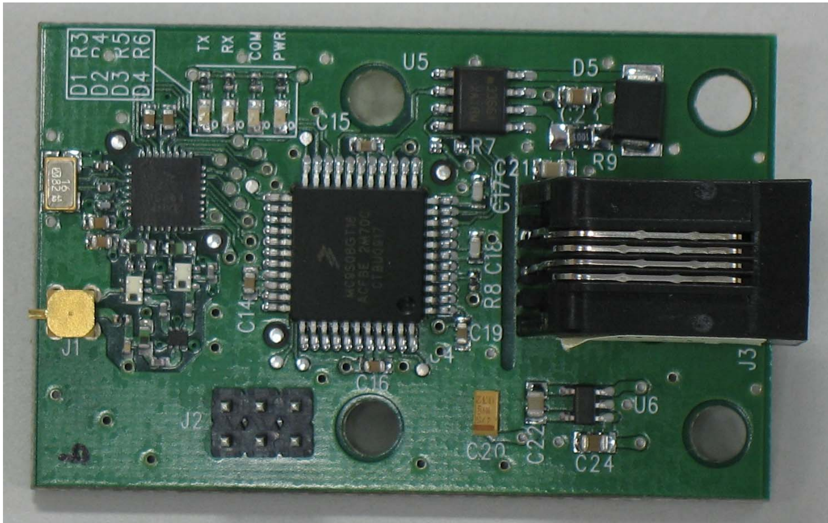
Transceiver Board, Component Side
