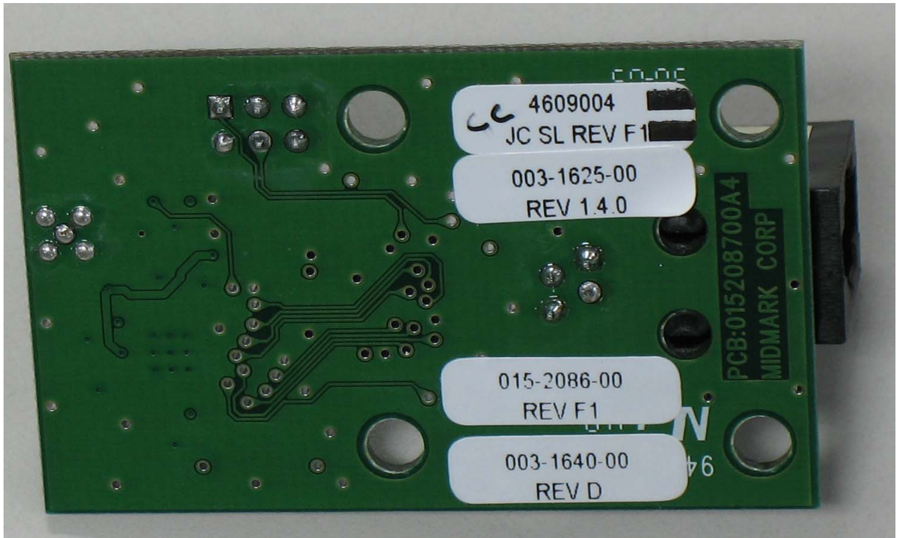
Transceiver Board, Solder Side
