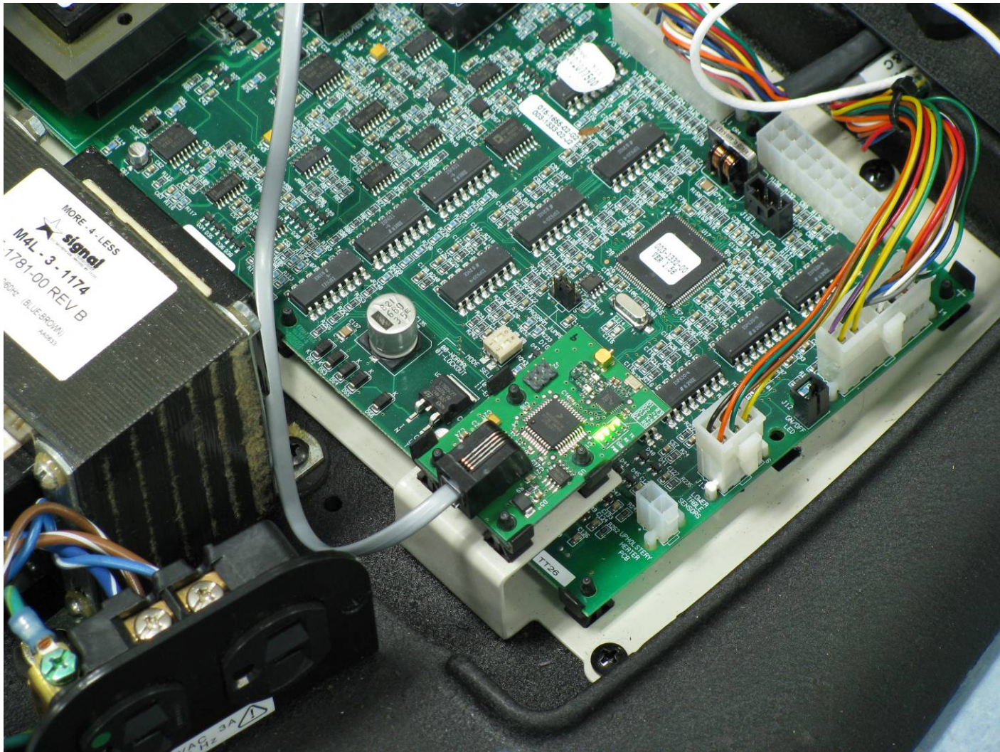
Cover Removed, Zoomed in on Transceiver
