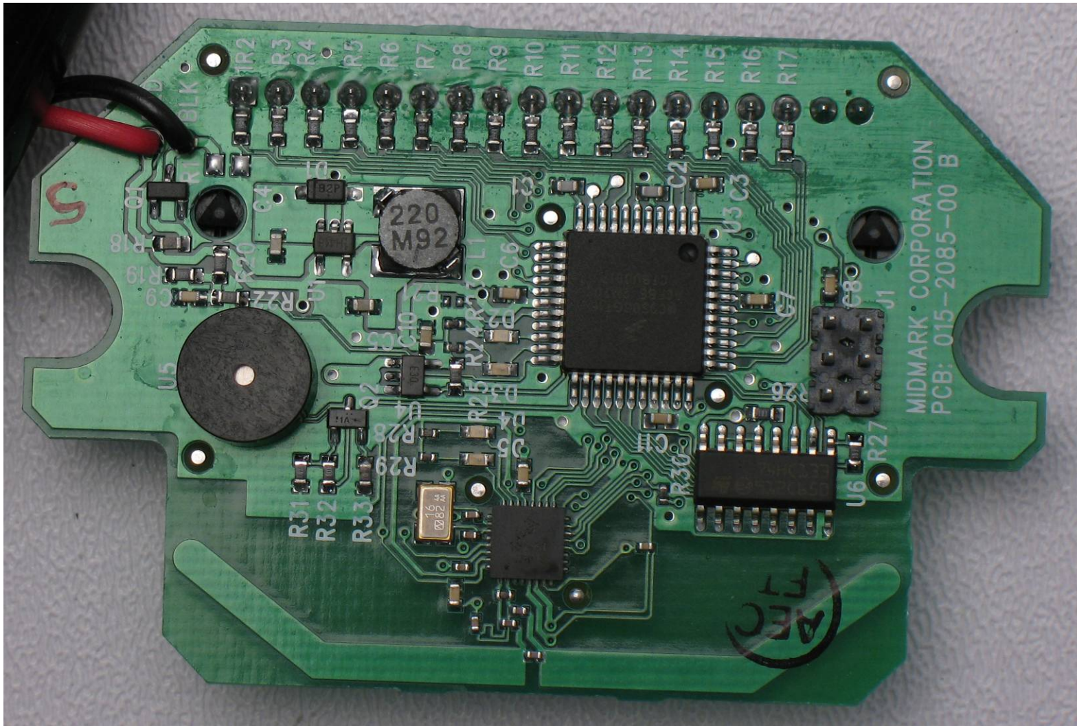
Circuit Board, Component Side
