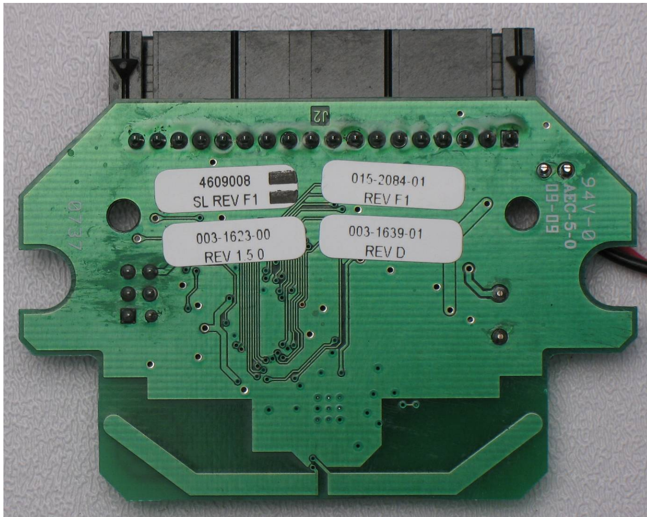
Circuit Board, Solder Side
