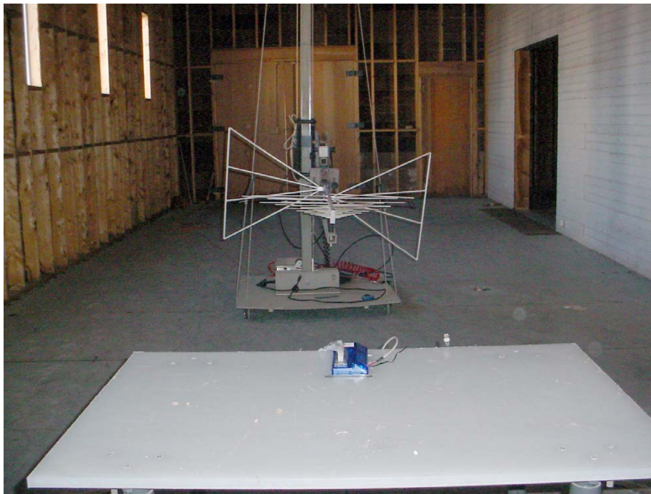
Radiated Emission at 3 m Distance
