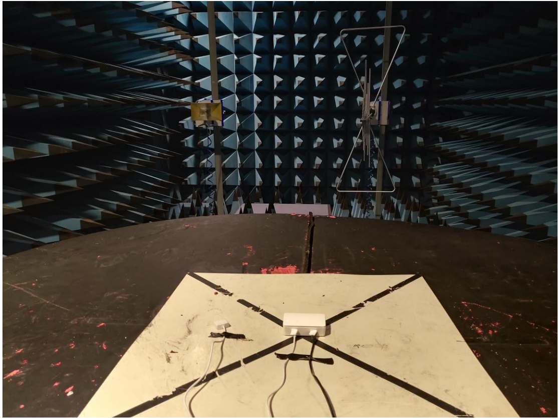
Radiated Emission above 1-18GHz
