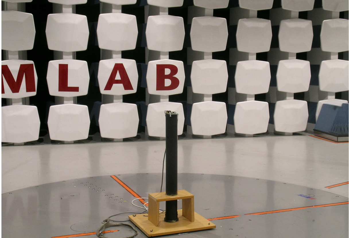
Radiated Emissions Measurement
