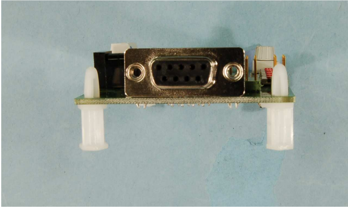
View of RS 232 port on the demonstration board
