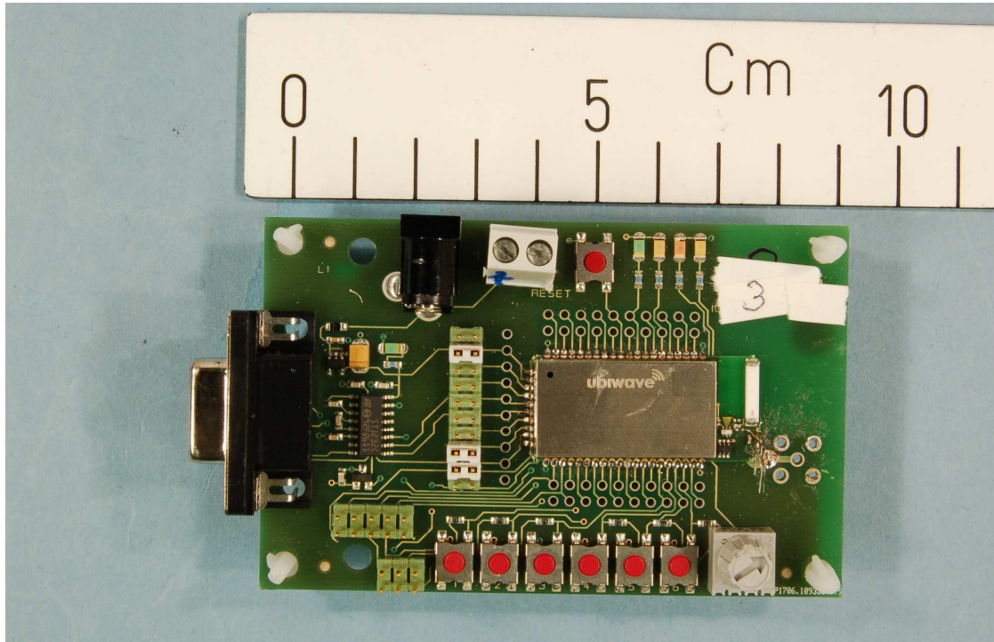
Demonstration board (as host) where the EUT is mounted during all tests
