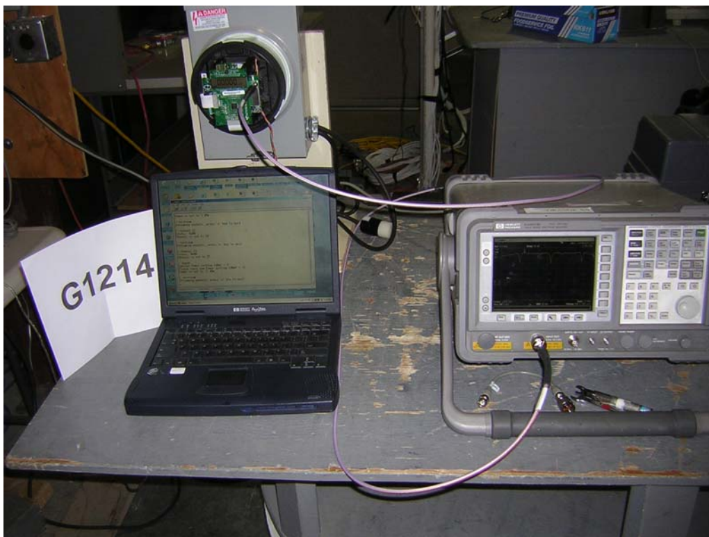
Conducted spurious emissions, POP, and PSD measurements
