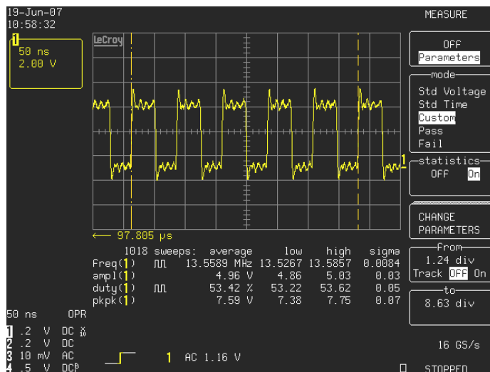
Figure 1.4 TX1 Output, No Load
