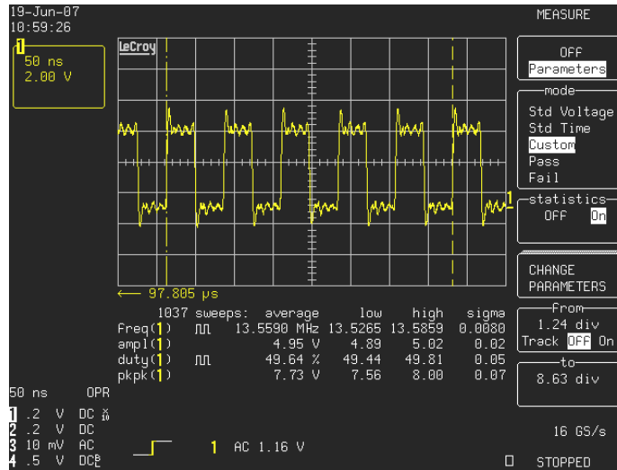
Figure 1.5 TX2 Output, No Load
