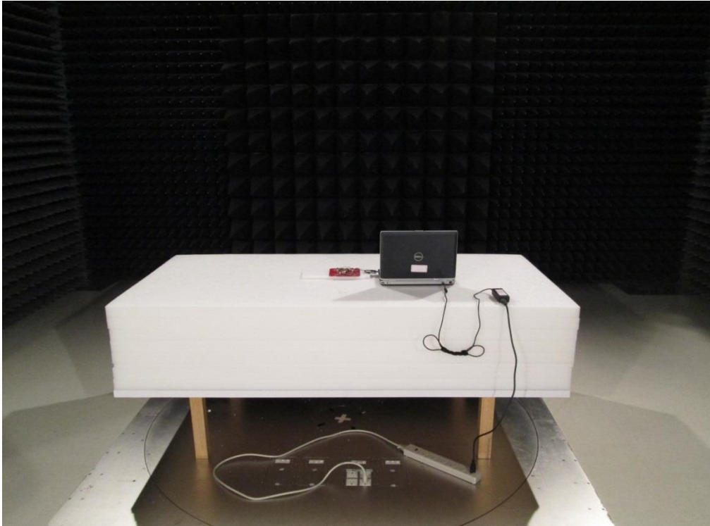
Radiated Test_Ant 3
