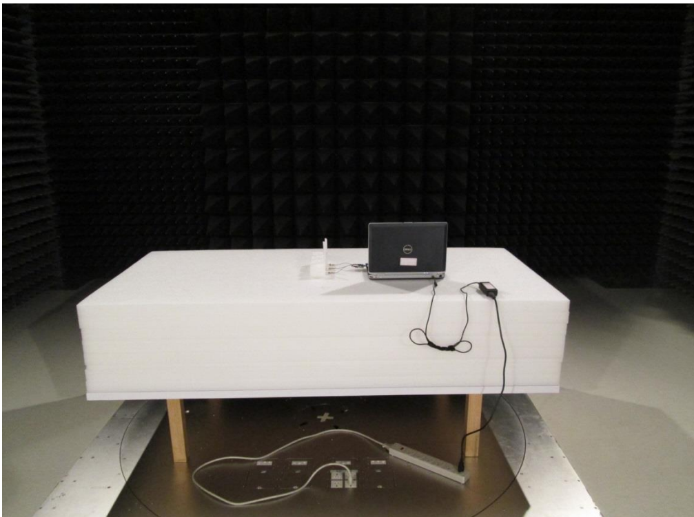
Radiated Test_Ant 2
