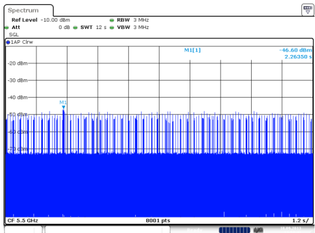
Calibration Radar #1 detection threshold level
