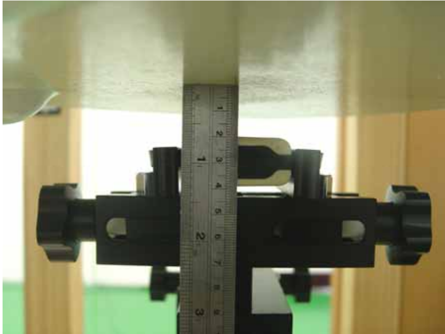
Fig. 9.1 Keypad Up with 2cm Gap
