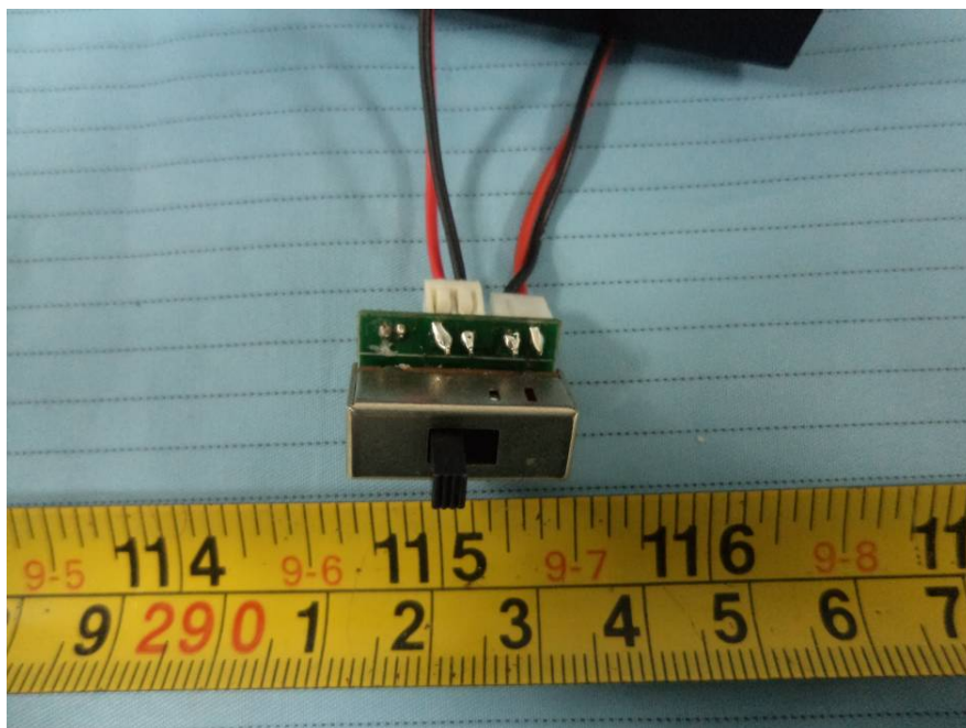
EUT – Battery Switch Board Top View
