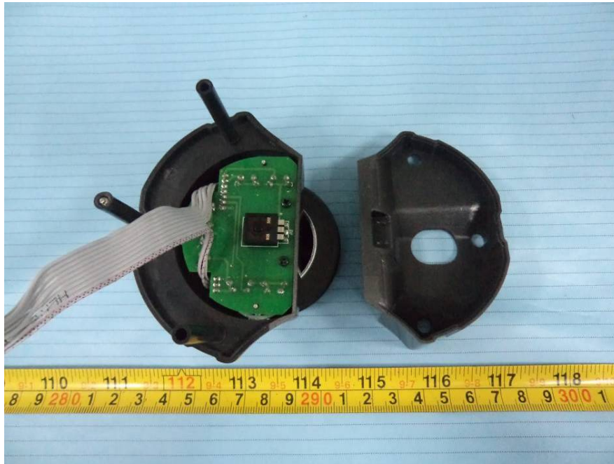
EUT – Wheel Cover off View
