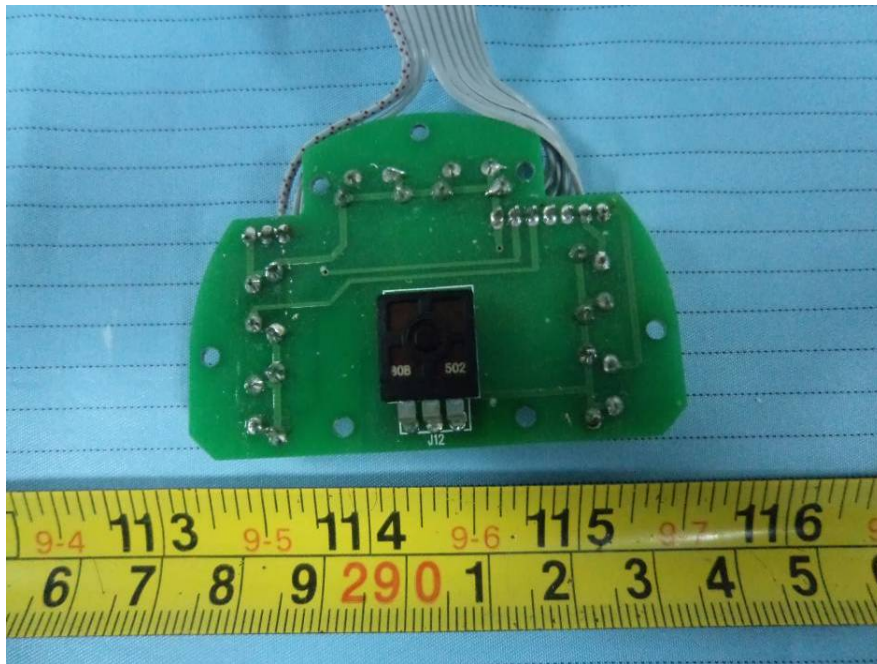
EUT – Wheel Board Bottom View
