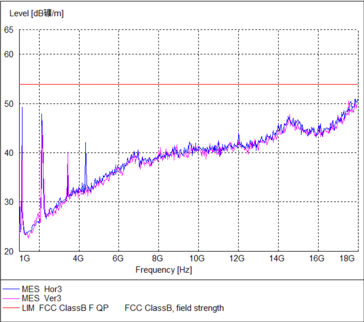
Plot of Radiation Emissions Test (Above 1GHz)
