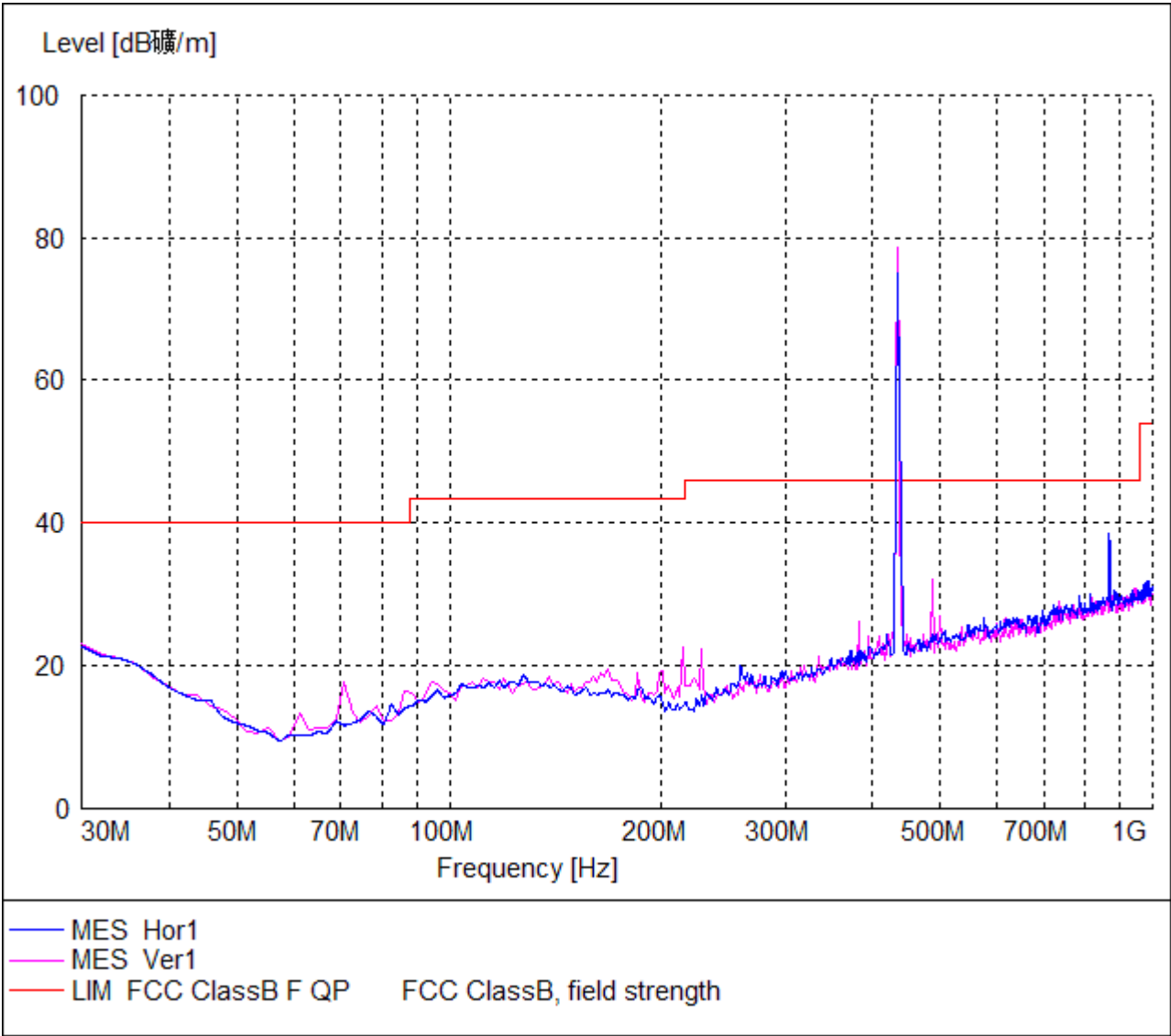
Plot of Radiation Emissions Test (Below 1GHz)
