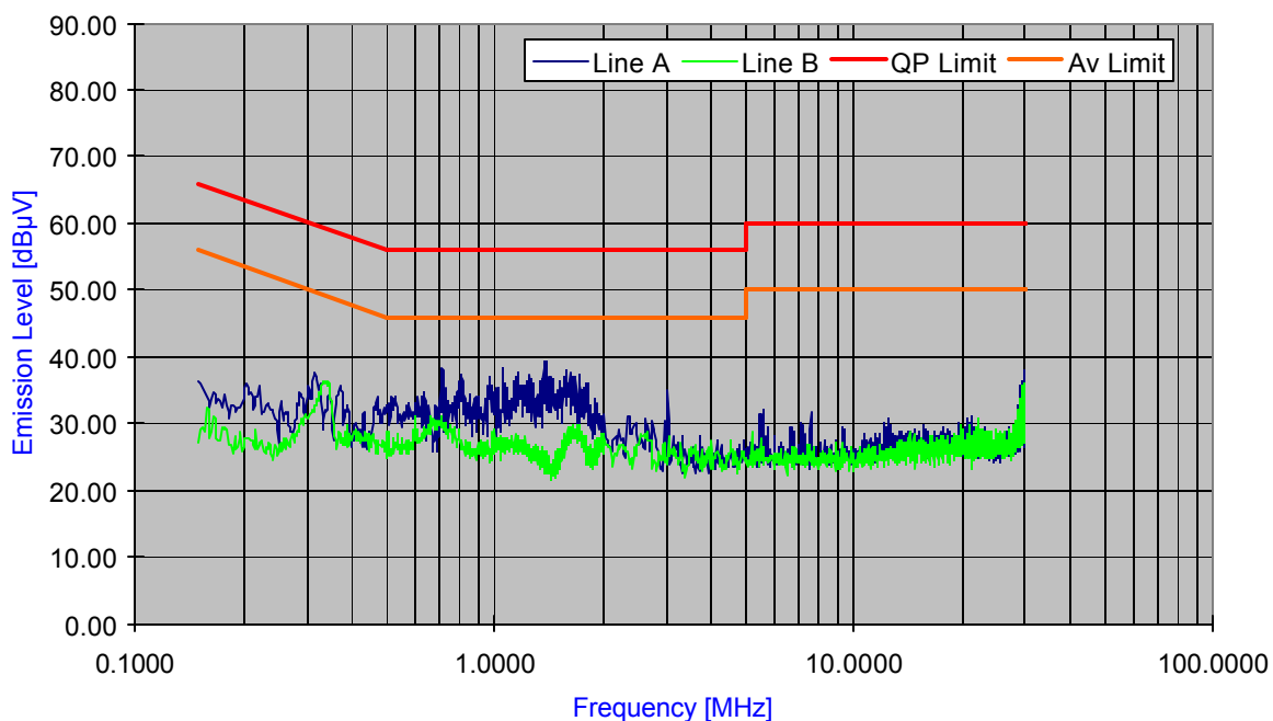
Plot 6-18. Line Conducted Plot with Bluetooth
