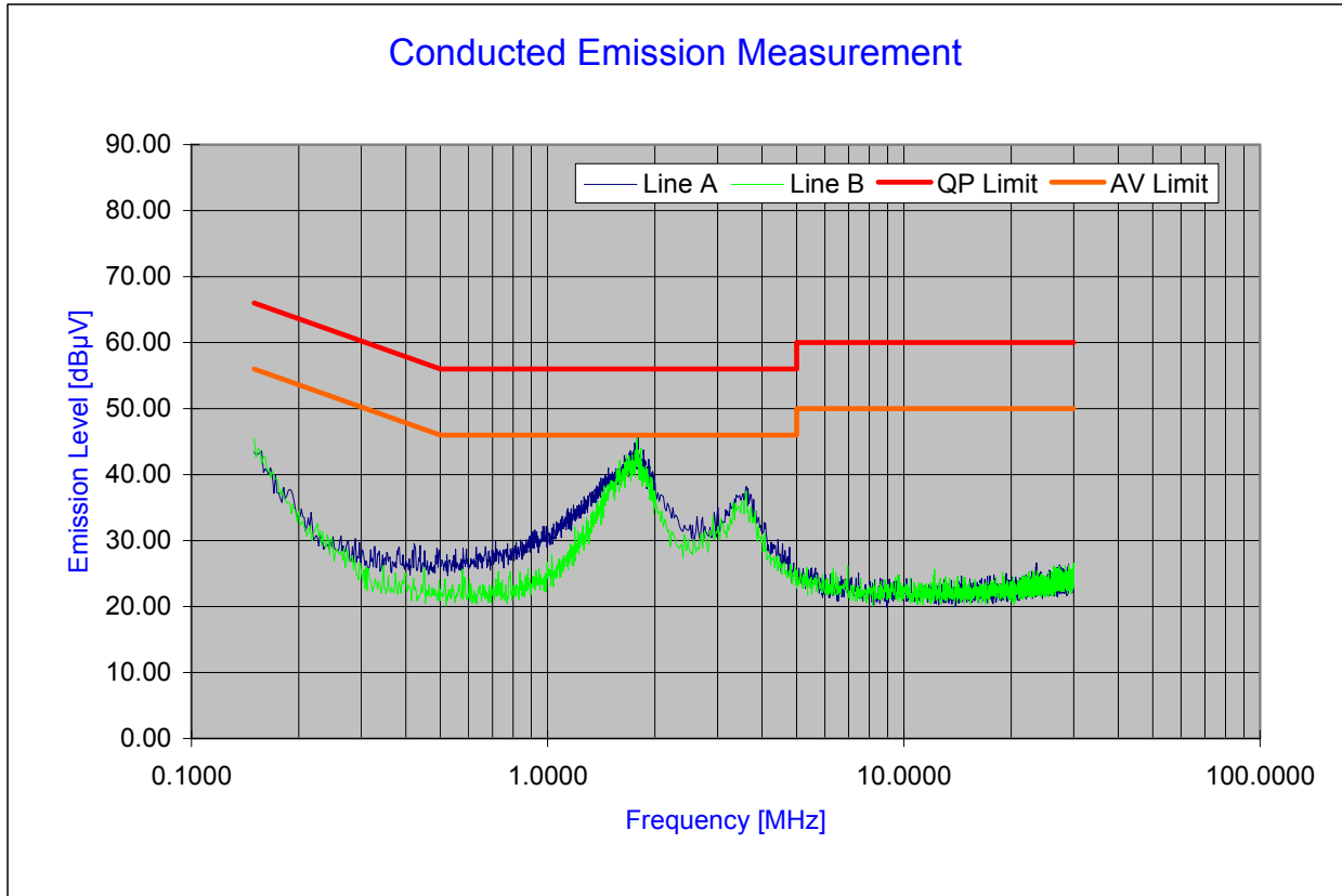
Plot 8-2. Line-Conducted Test Plot (RFID Antenna Terminated)
