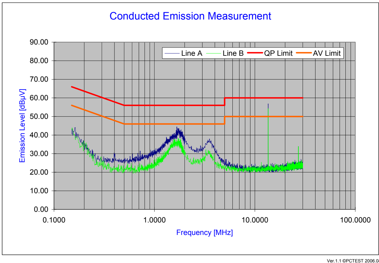
Plot 8-1. Line-Conducted Test Plot (RFID Antenna Active)
