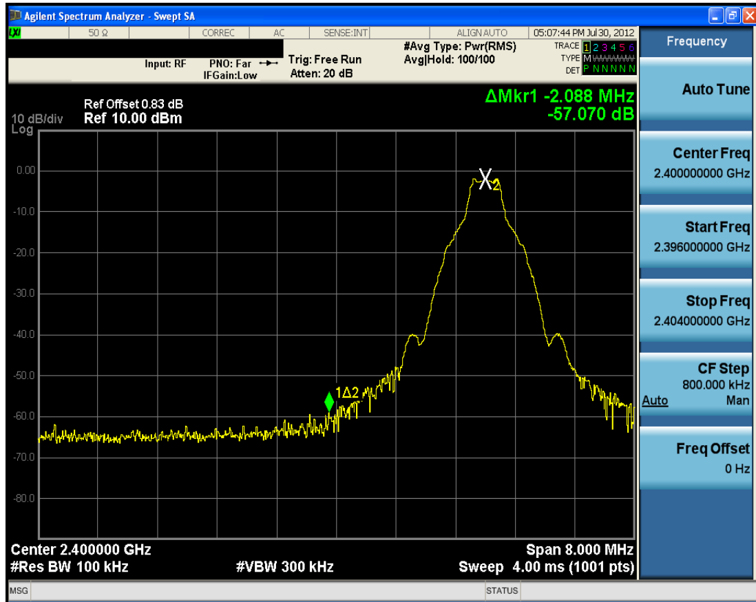
Plot 6-10. Band Edge Plot (Bluetooth with Hopping Disabled, 1Mbps – Ch. 0)
