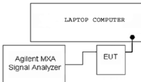
Figure 6-3. Test Instrument & Measurement Setup
