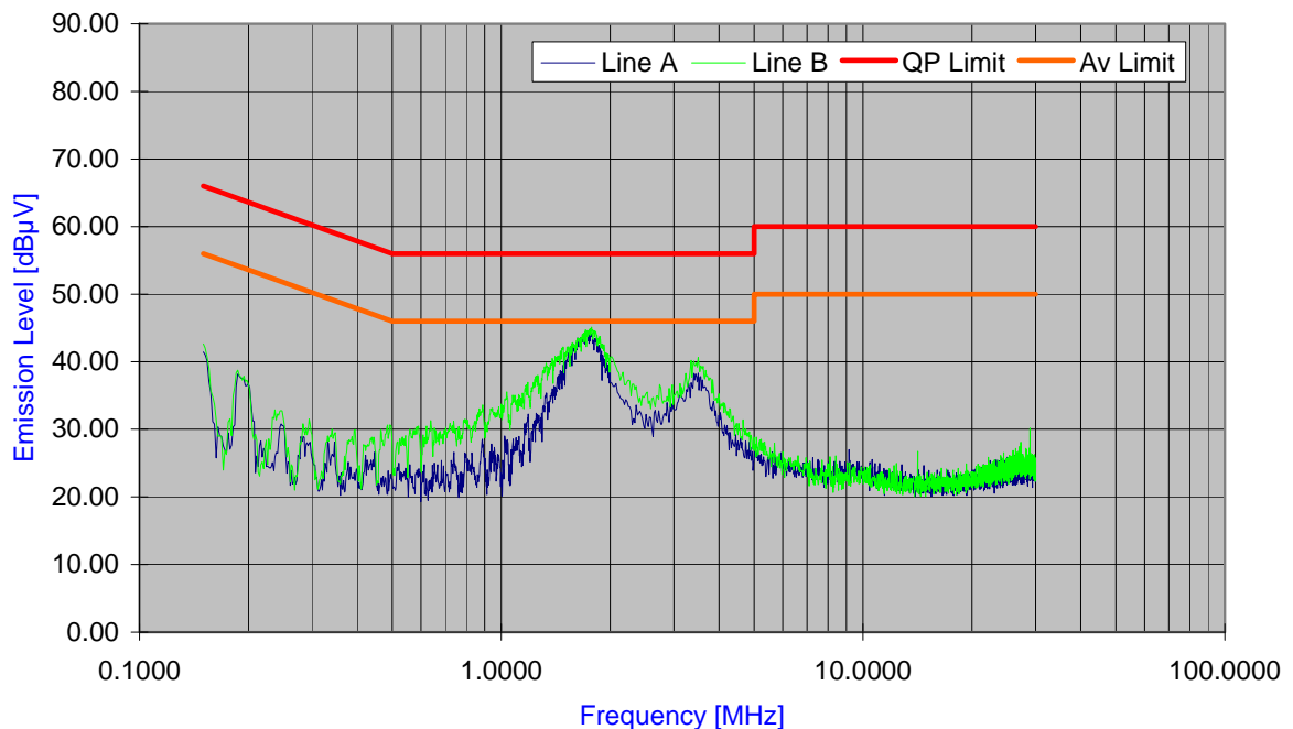
Plot 6-15. Line Conducted Plot with Bluetooth (LE)
