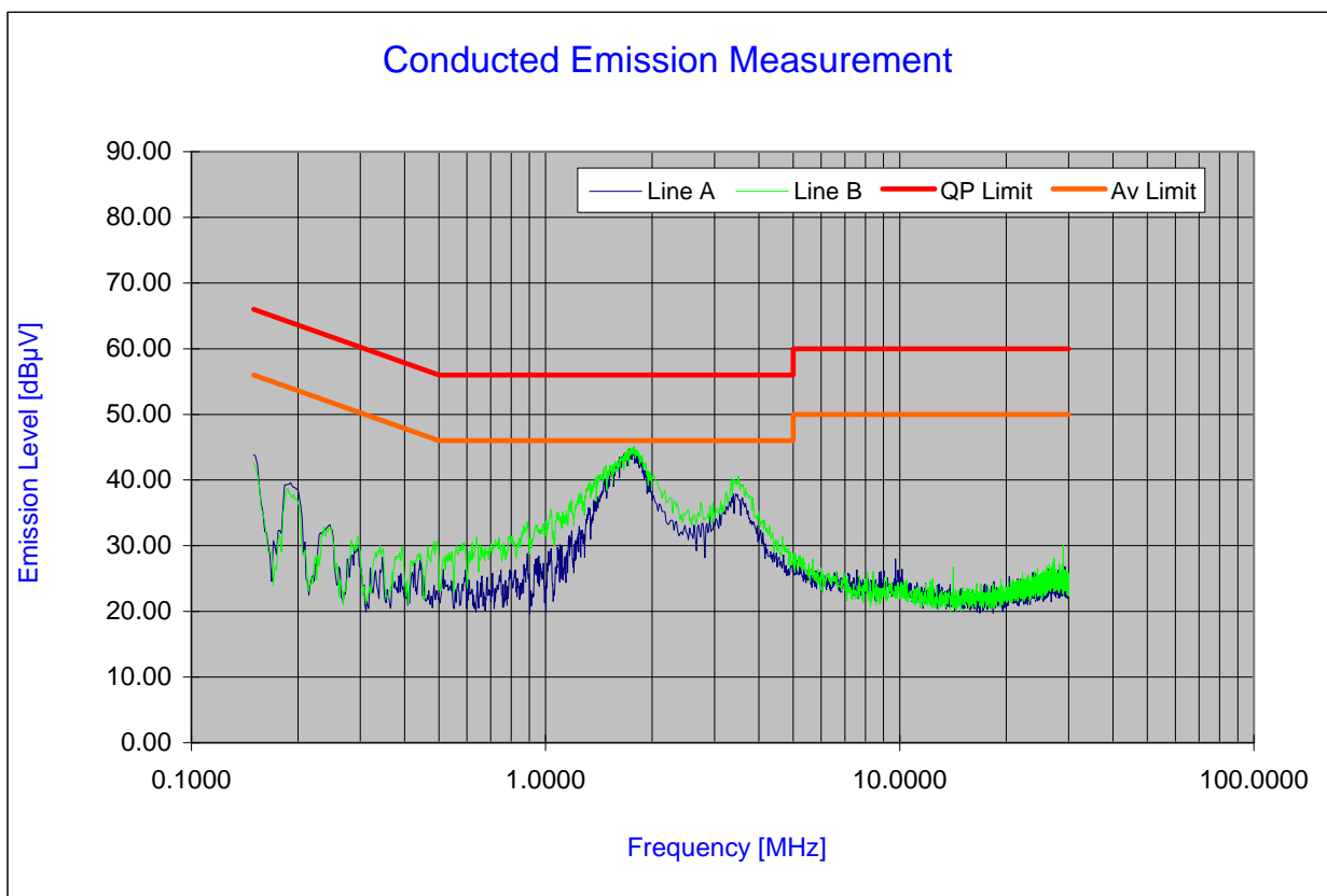
Plot 6-31. Line Conducted Plot with 802.11b
