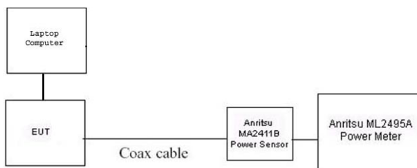
Figure 6-2. Test Instrument & Measurement Setup
