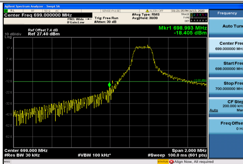
Band12-3MHz-QPSK-23025-1RB#0
