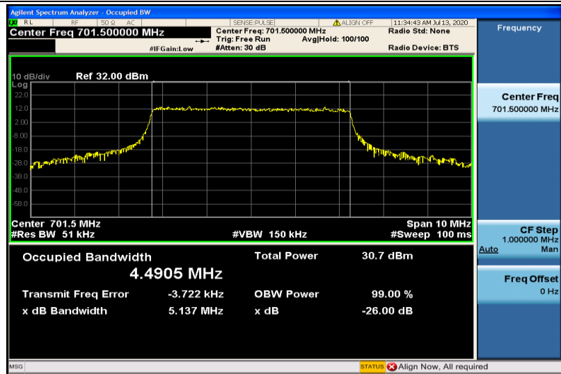
Band12-5MHz-16QAM-23035-25RB#0-4.4905
