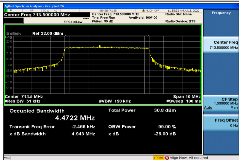
Band12-5MHz-16QAM-23155-25RB#0-4.4722
