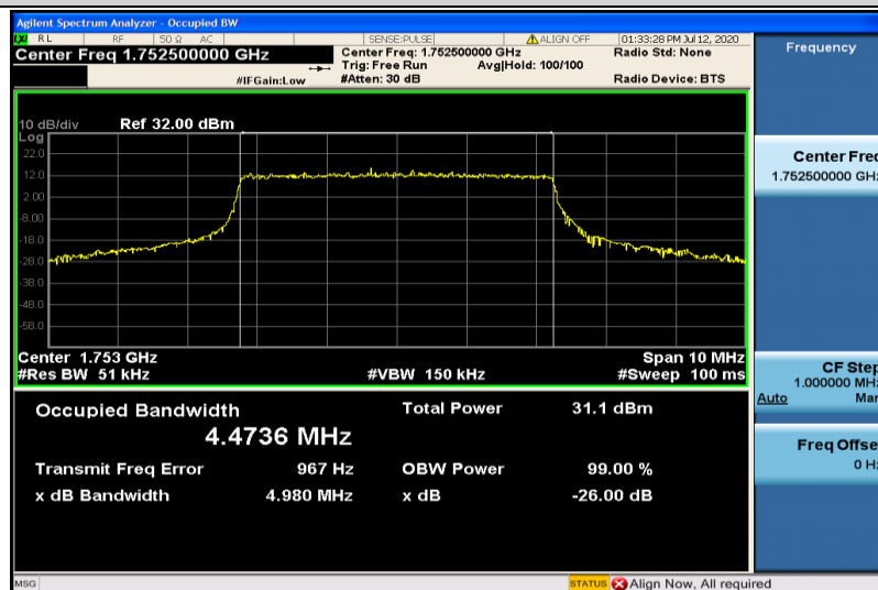
Band4-5MHz-16QAM-20375-25RB#0-4.4736
