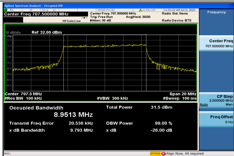
Band12-10MHz-QPSK-23095-50RB#0-8.9513
