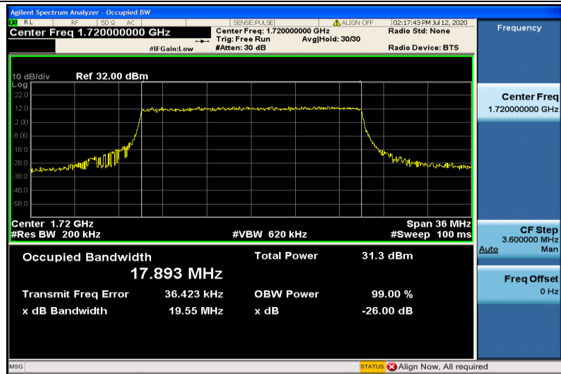
Band4-20MHz-16QAM-20050-100RB#0-17.893
