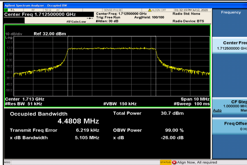
Band4-5MHz-16QAM-19975-25RB#0-4.4808
