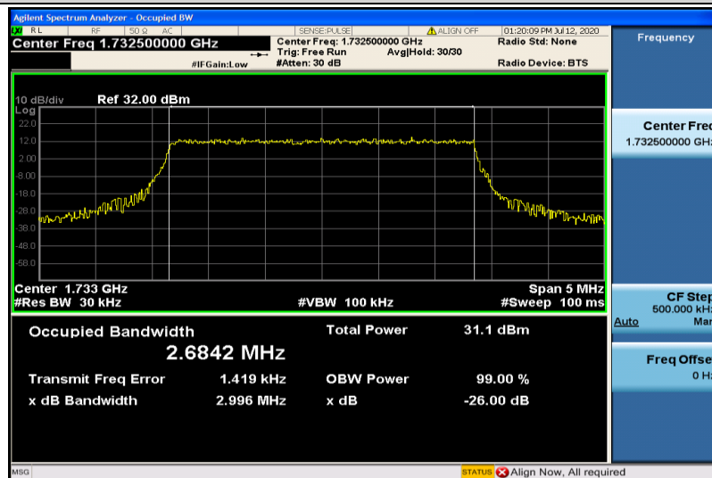
Band4-3MHz-QPSK-20175-15RB#0-2.6842
