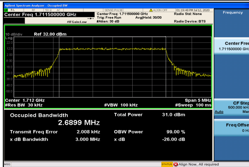
Band4-3MHz-QPSK-19965-15RB#0-2.6899
