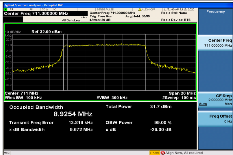
Band12-10MHz-QPSK-23130-50RB#0-8.9254
