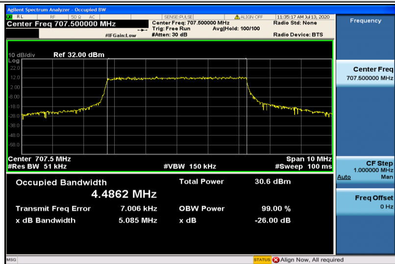
Band12-5MHz-16QAM-23095-25RB#0-4.4862
