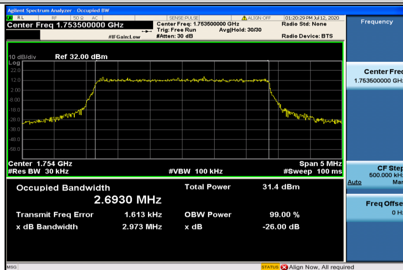
Band4-3MHz-QPSK-20385-15RB#0-2.6930
