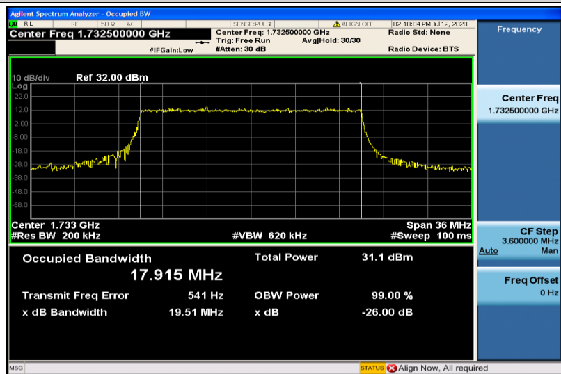
Band4-20MHz-16QAM-20175-100RB#0-17.915
