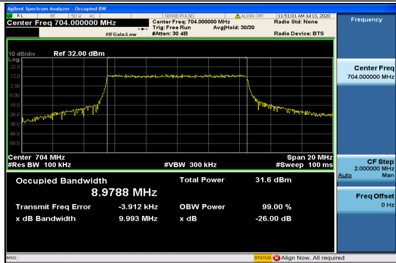
Band12-10MHz-QPSK-23060-50RB#0-8.9788
