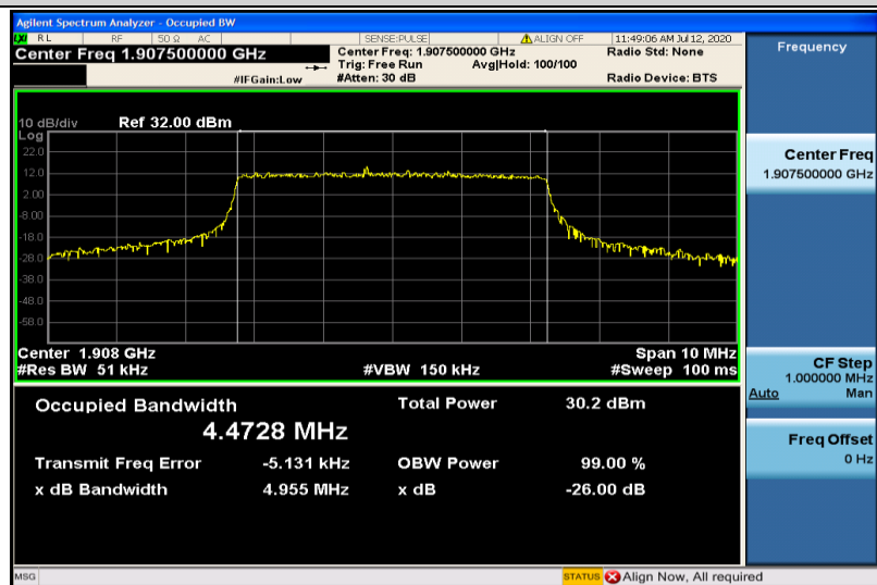
Band2-5MHz-16QAM-19175-25RB#0-4.4728
