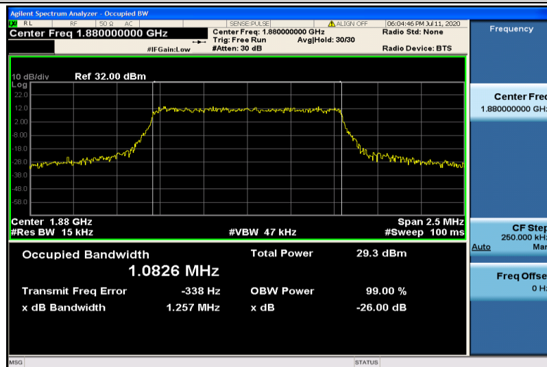
Band2-1.4MHz-16QAM-18900-6RB#0-1.0826
