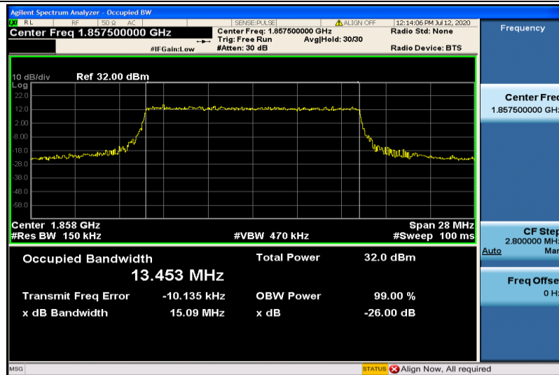
Band2-15MHz-QPSK-18675-75RB#0-13.453
