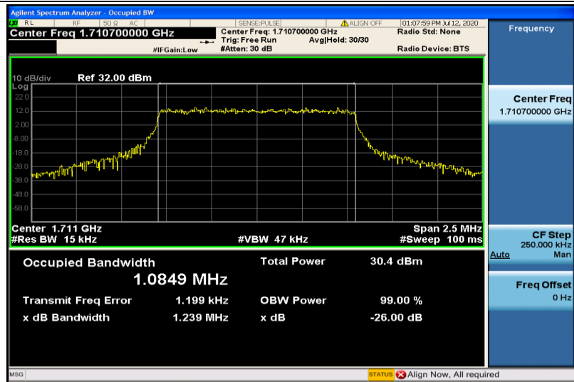
Band4-1.4MHz-QPSK-19957-6RB#0-1.0849
