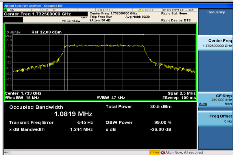
Band4-1.4MHz-QPSK-20175-6RB#0-1.0819
