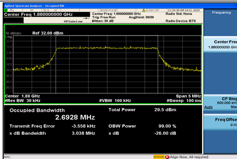
Band2-3MHz-16QAM-18900-15RB#0-2.6928
