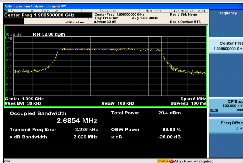
Band2-3MHz-16QAM-19185-15RB#0-2.6854
