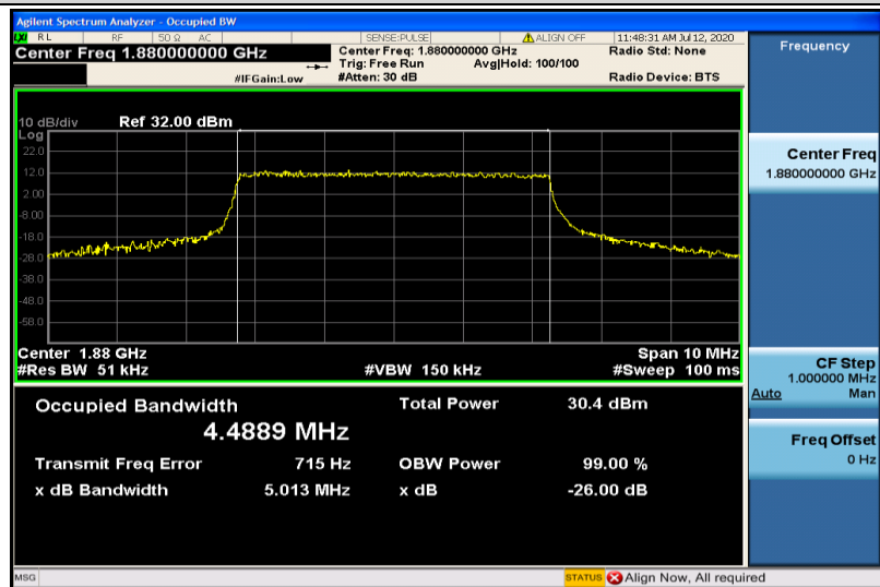
Band2-5MHz-16QAM-18900-25RB#0-4.4889
