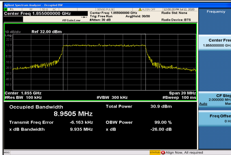
Band2-10MHz-16QAM-18650-50RB#0-8.9505
