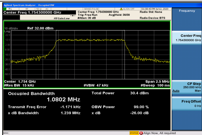
Band4-1.4MHz-QPSK-20393-6RB#0-1.0802
