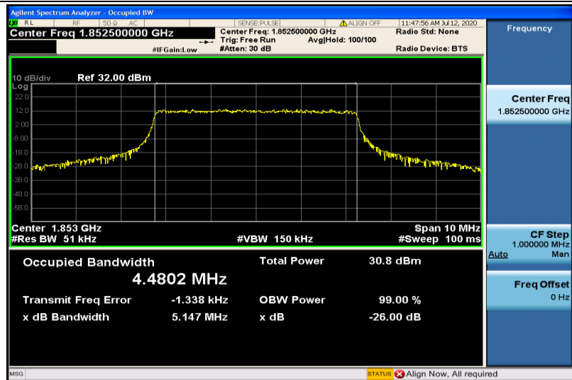
Band2-5MHz-16QAM-18625-25RB#0-4.4802
