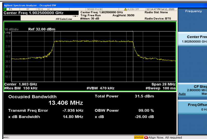
Band2-15MHz-QPSK-19125-75RB#0-13.406
