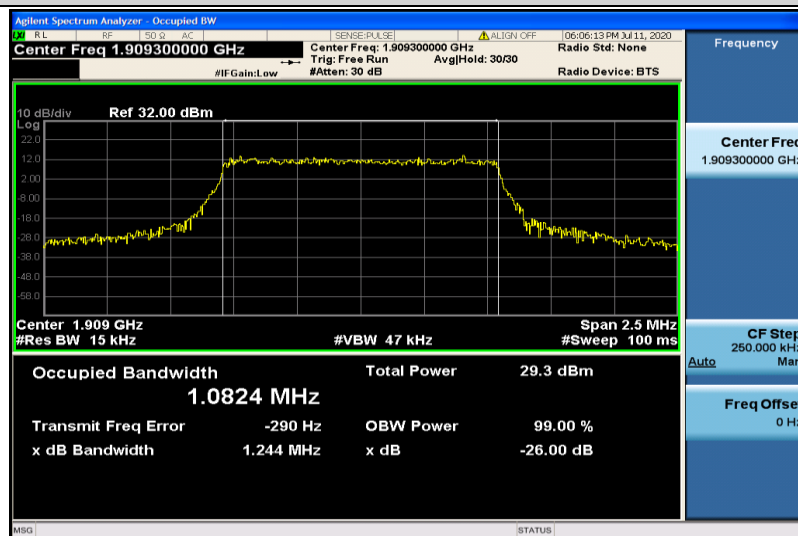
Band2-1.4MHz-16QAM-19193-6RB#0-1.0824
