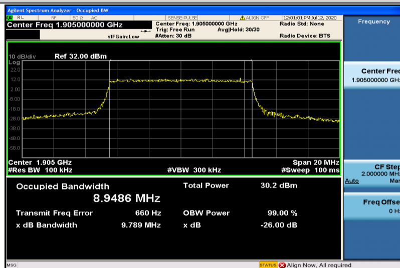
Band2-10MHz-16QAM-19150-50RB#0-8.9486
