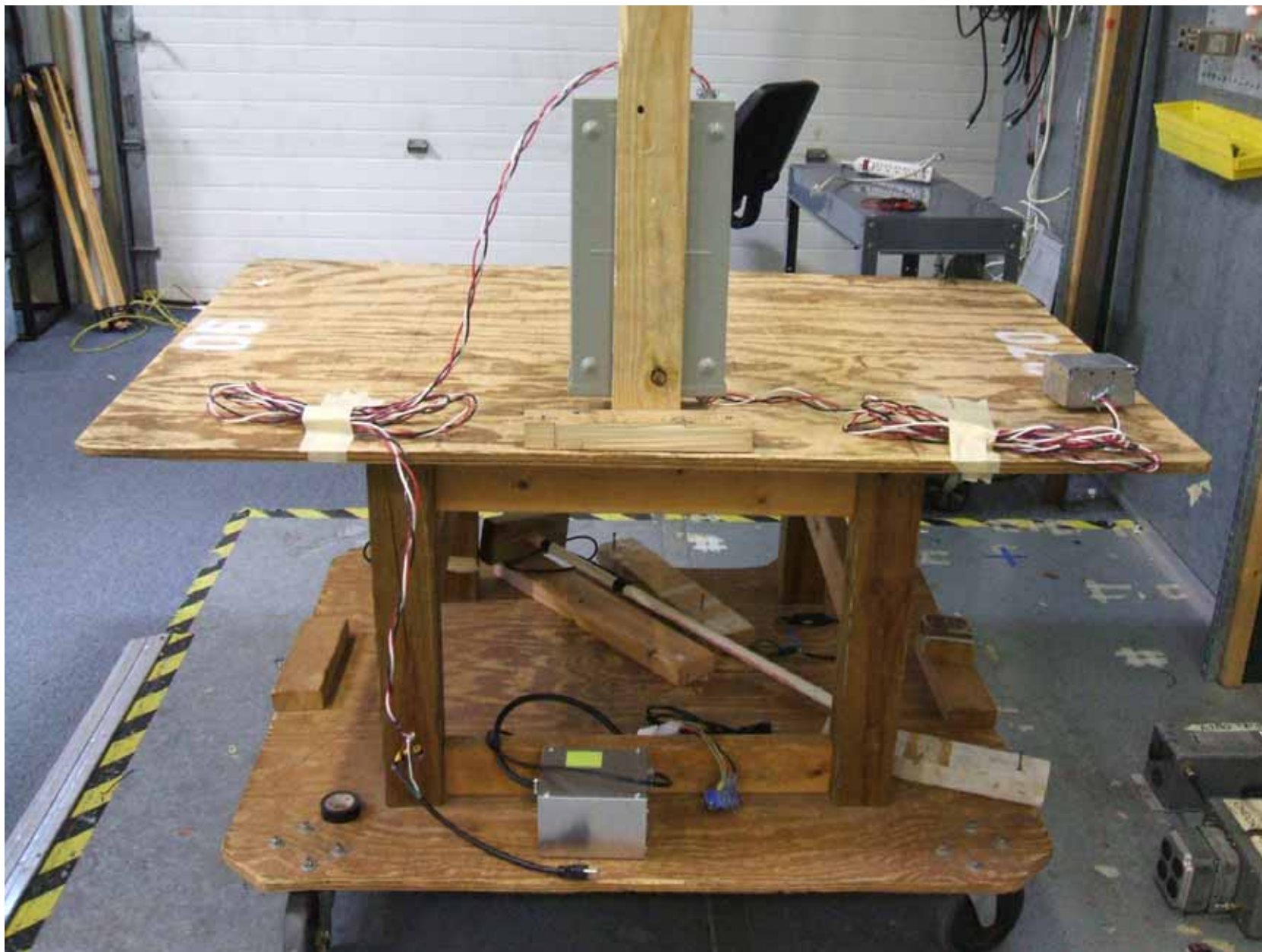
Photograph B-2: Conducted Emissions Test and Radiated Emissions Test – Washington Laboratories – Rear View
