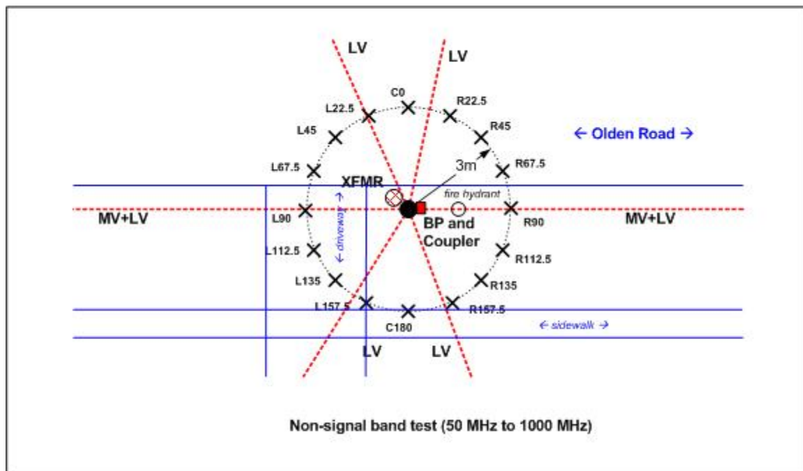
Figure 3: Test Site Diagram – CURRENT Technologies Rockville Test Area – BP-02
