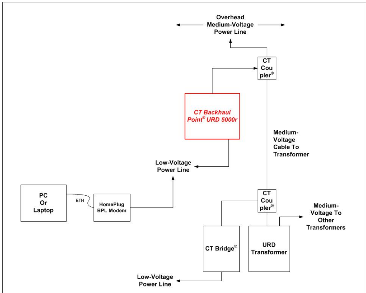
Figure 1: System Test Configuration
