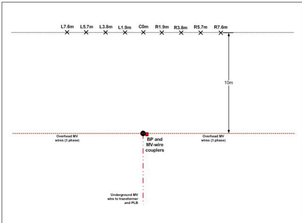
Figure 10: Test Site Diagram – CURRENT Technologies Field Research and Test Area – P3
