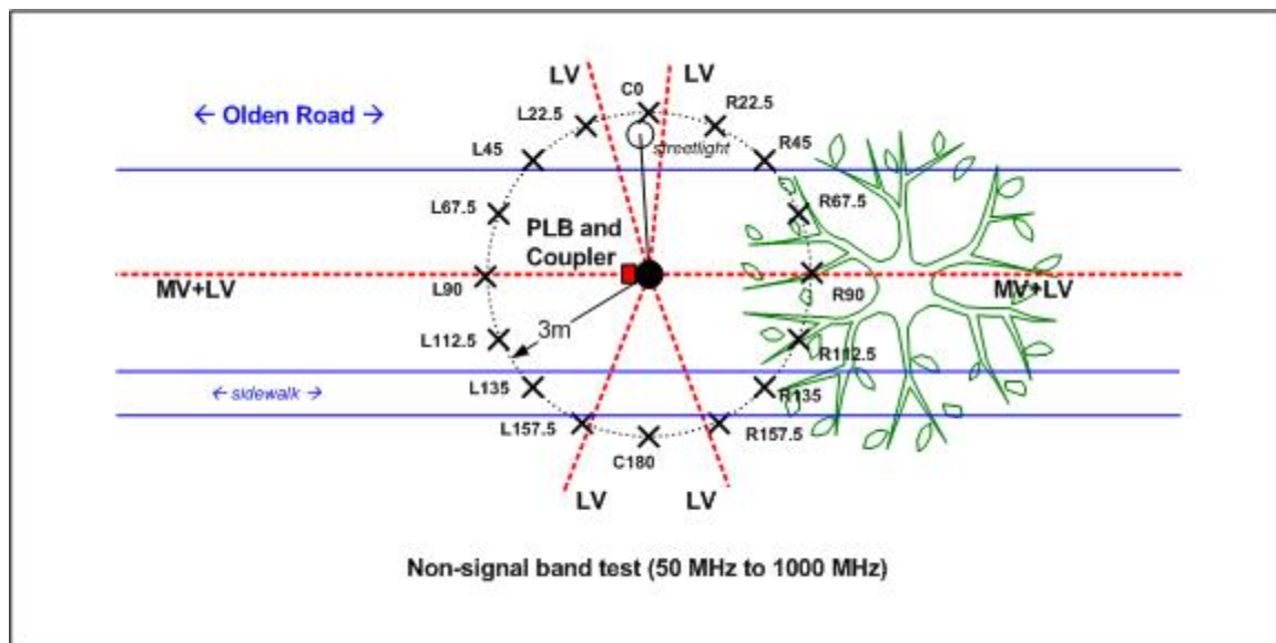
Figure 4: Test Site Diagram – CURRENT Technologies Rockville Test Area – BP-03
