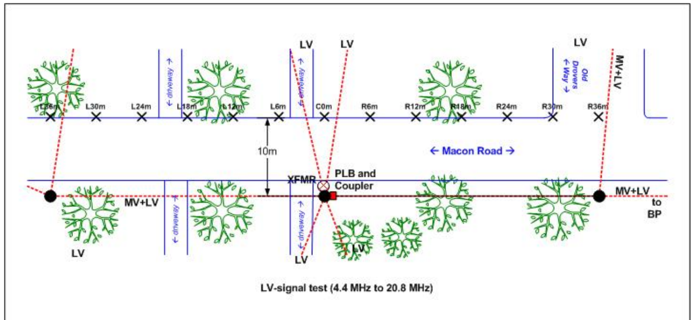
Figure 6: Test Site Diagram – CURRENT Technologies Rockville Test Area – PLB-02
