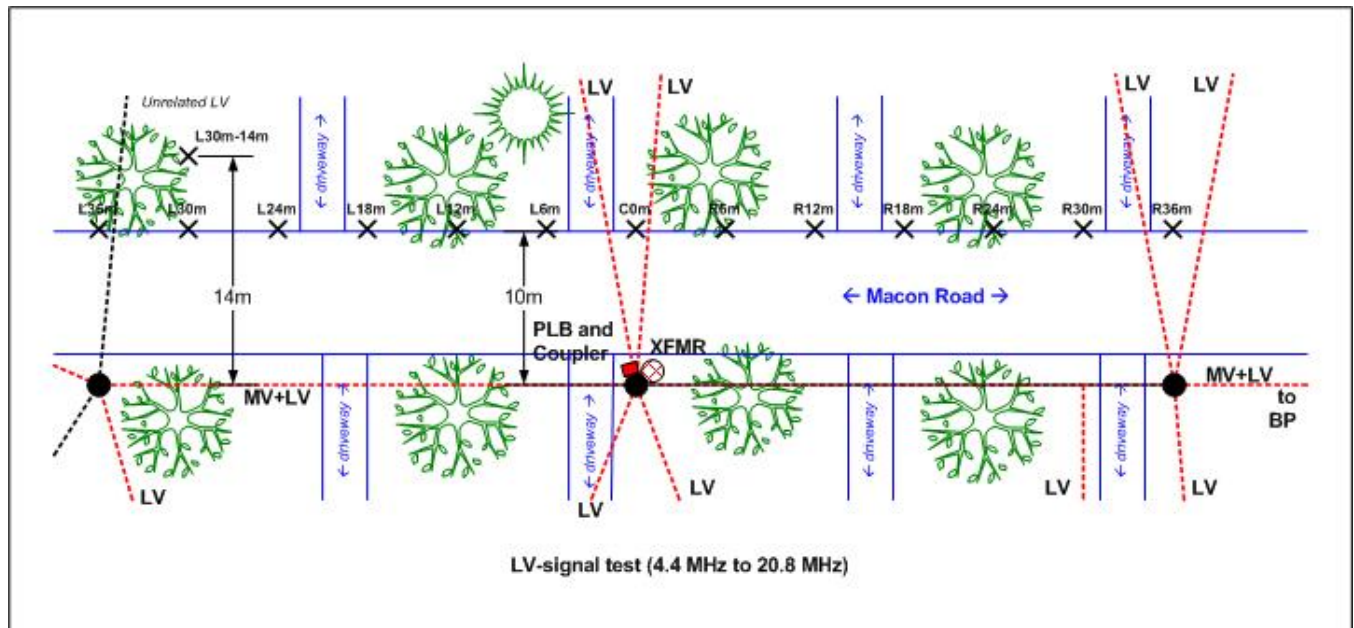
Figure 5: Test Site Diagram – CURRENT Technologies Rockville Test Area – PLB-01
