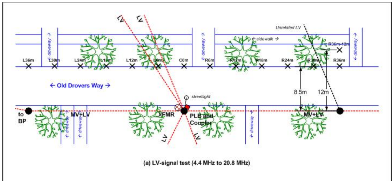
Figure 7: Test Site Diagram – CURRENT Technologies Rockville Test Area – PLB-04
