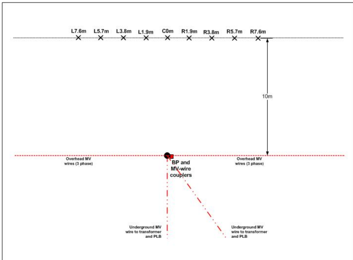
Figure 8: Test Site Diagram – CURRENT Technologies Field Research and Test Area – P4
