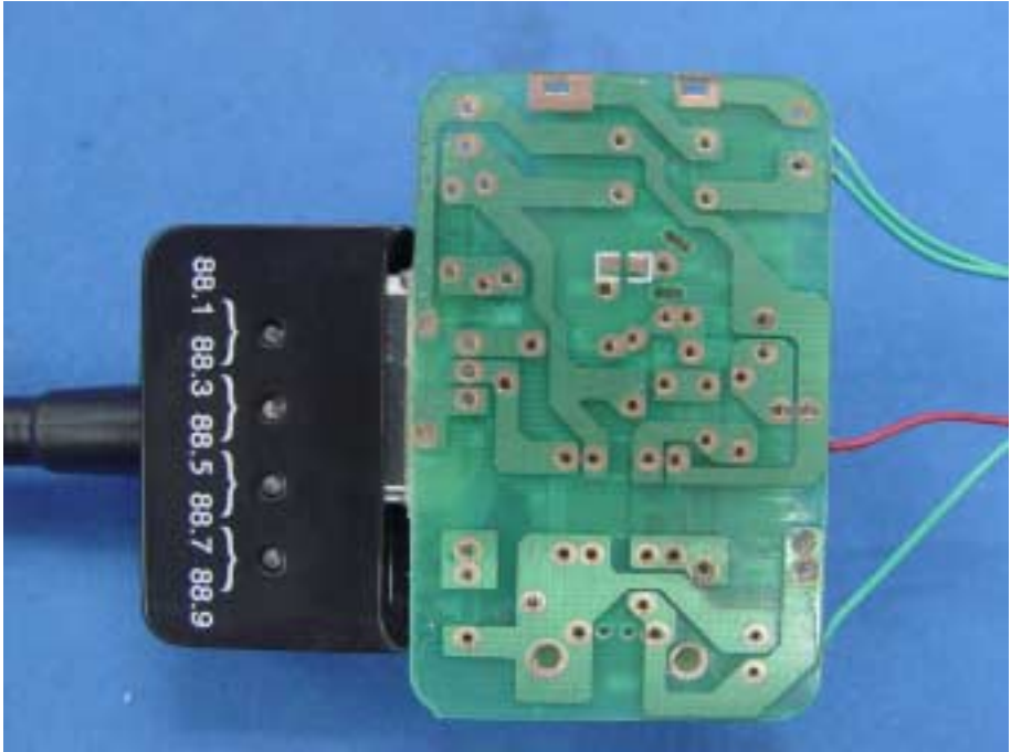
Figure 4 General Appearance
