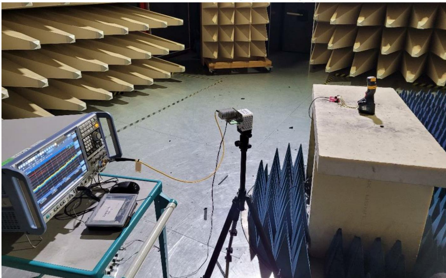
Anechoic chamber 18 GHz – 25 GHz
