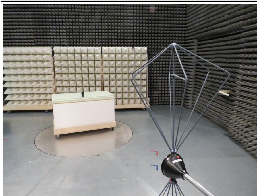
SETUP RADIATED EMISSION - 30MHz-200MHz
