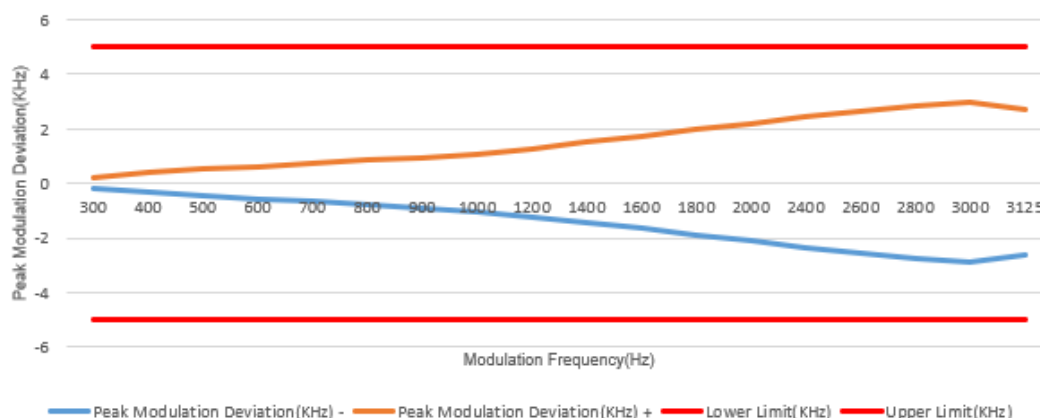
Audio Frequency Response
