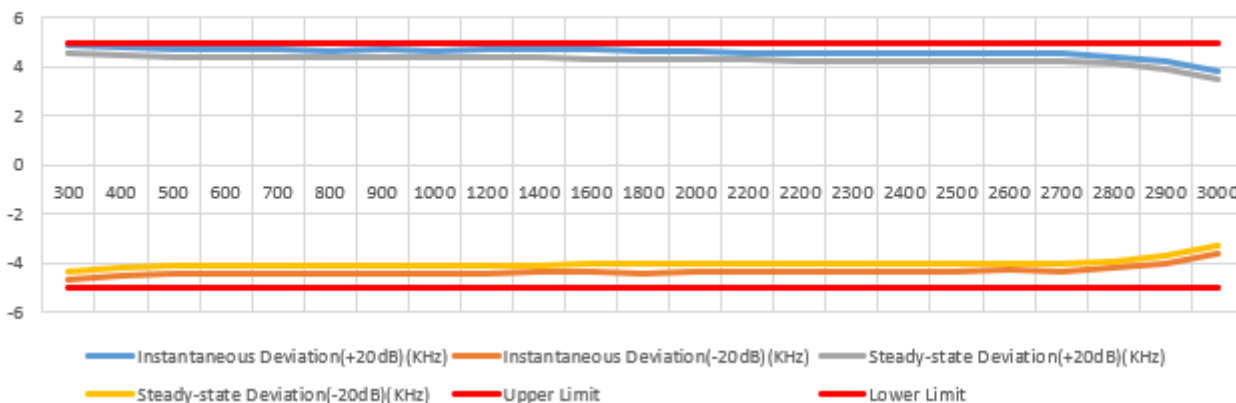
Modulation Limiting
