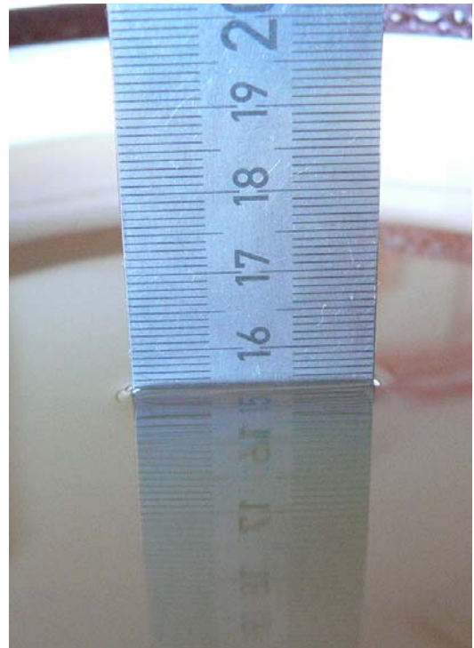
Fig. 19: Liquid depth for IEEE 802.11 a Body measurements
