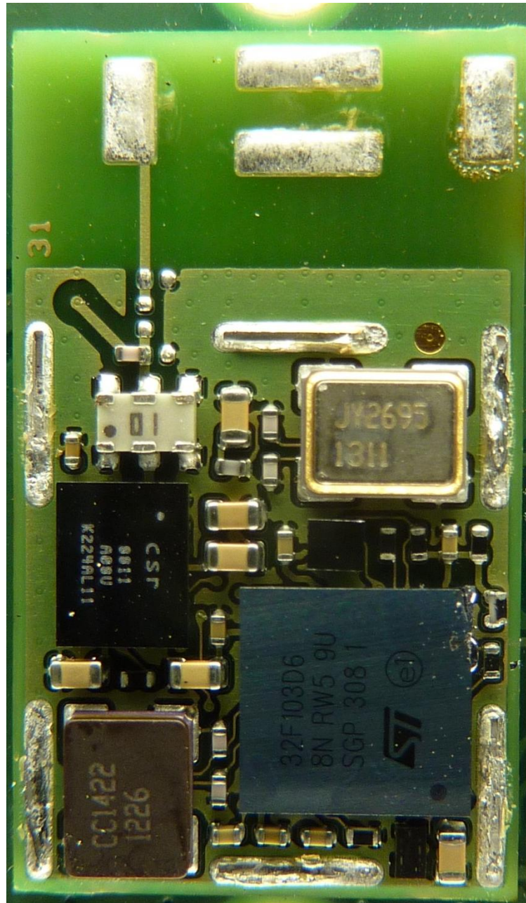
135190_8.JPG: Bluetooth module, detail view, shielding removed
