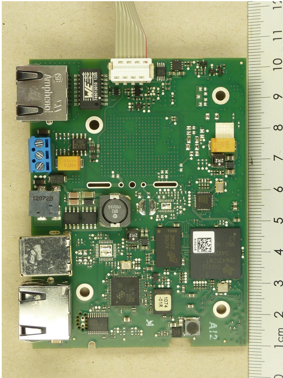
135190_6.JPG: Base Staion, Main PCB, bottom view
