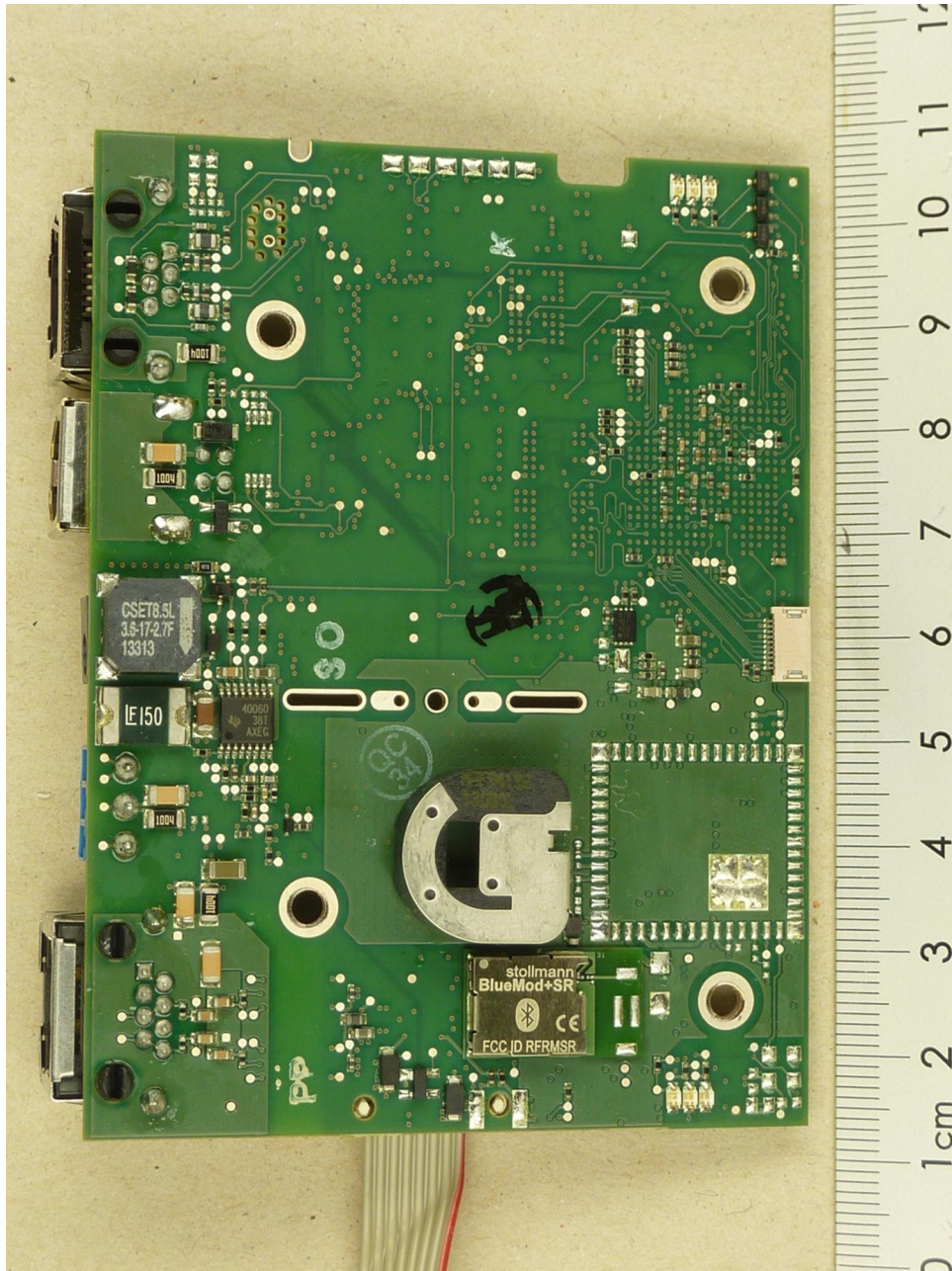
135190_5.JPG: Base Staion, Main PCB, top view
