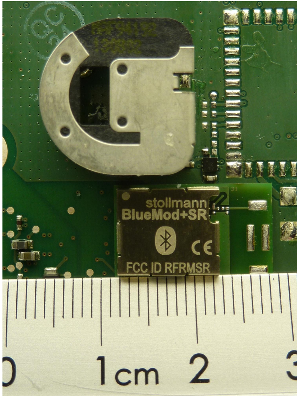
135190_7.JPG: Bluetooth module (shielded) and antenna
