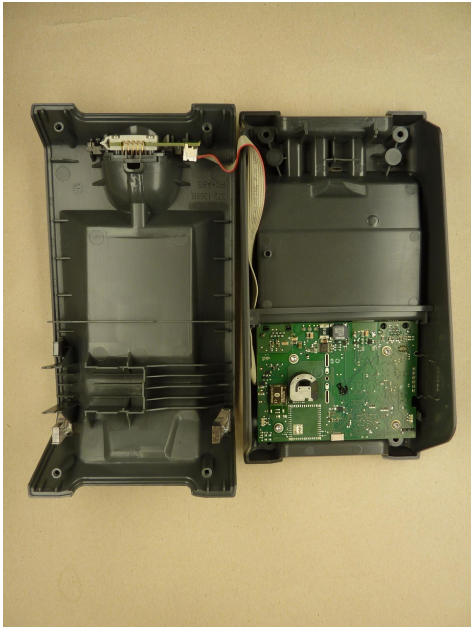
135190_4.JPG: Base Staion, internal view, location of PCB
