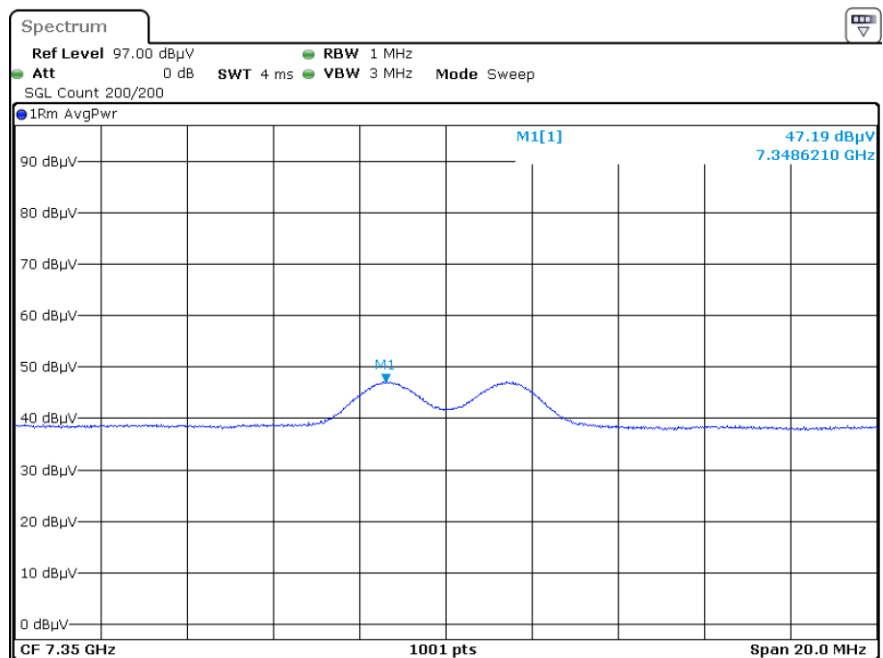
F2 X3 7350.0 Harmonic Vertical AVG
