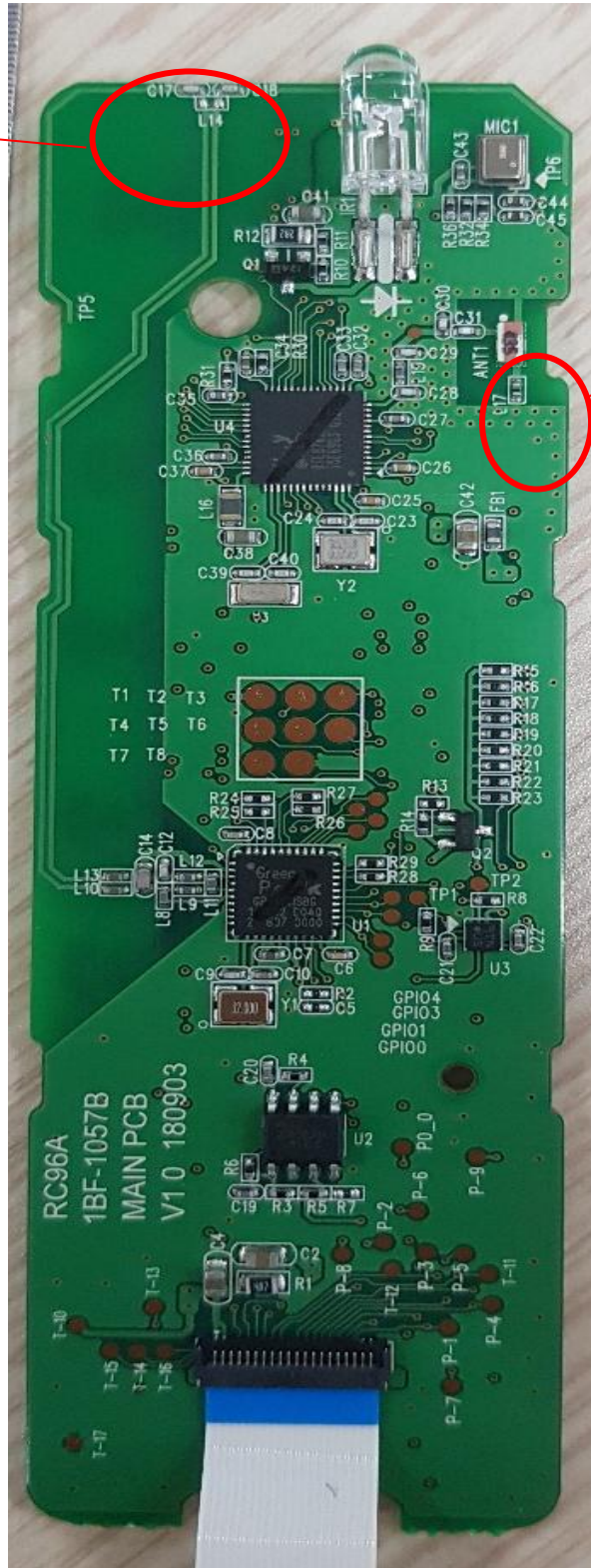
Antenna View
