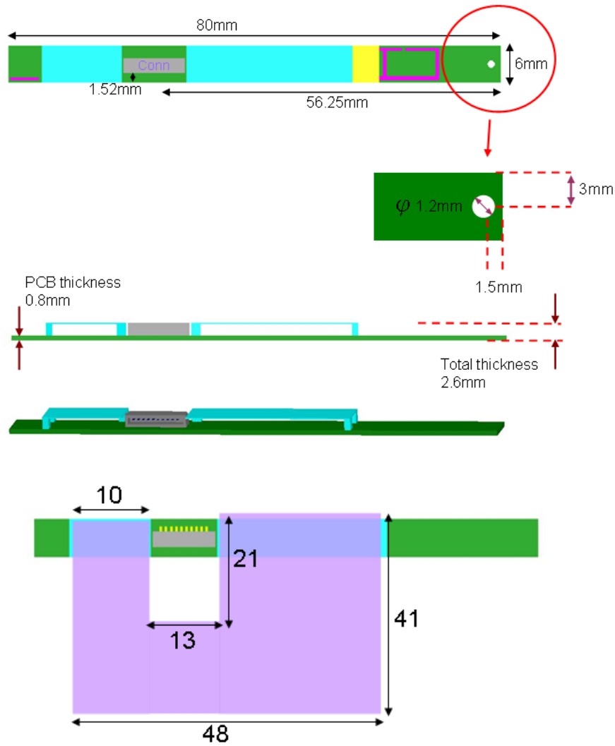
Figure 1. RTL8188CUS Slim Module Mechanical Specification
