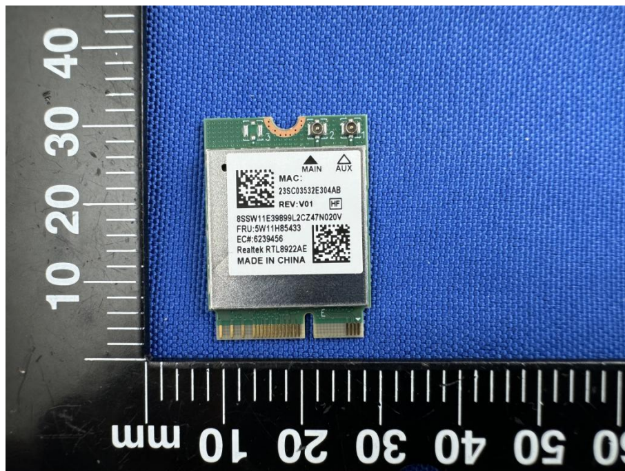
RF MODULE TOP VIEW -RTL8922AE (WITH SHIELDING)
