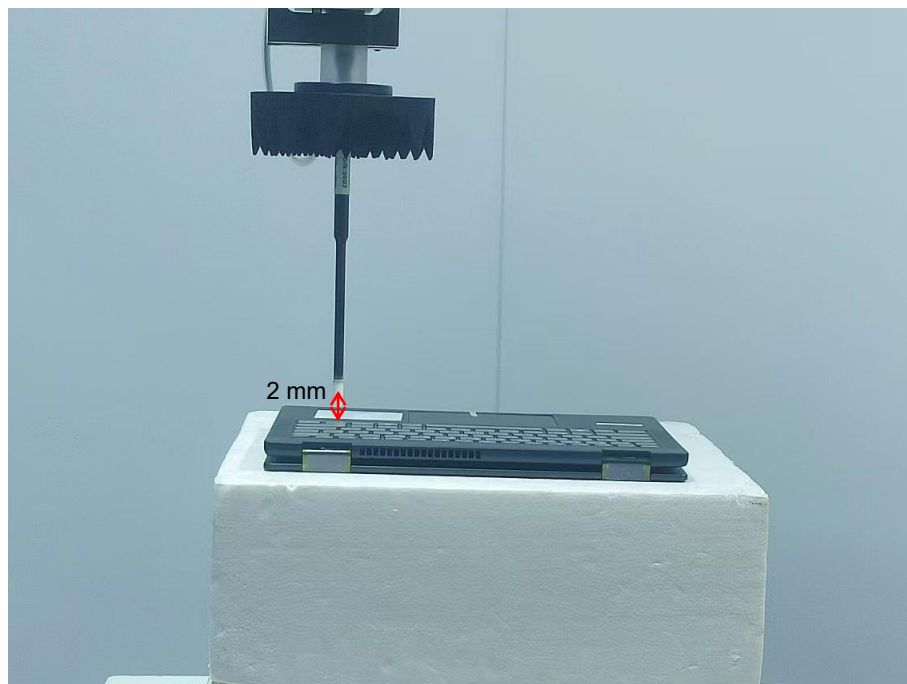
Keyboard Side (Tablet) (2mm)
