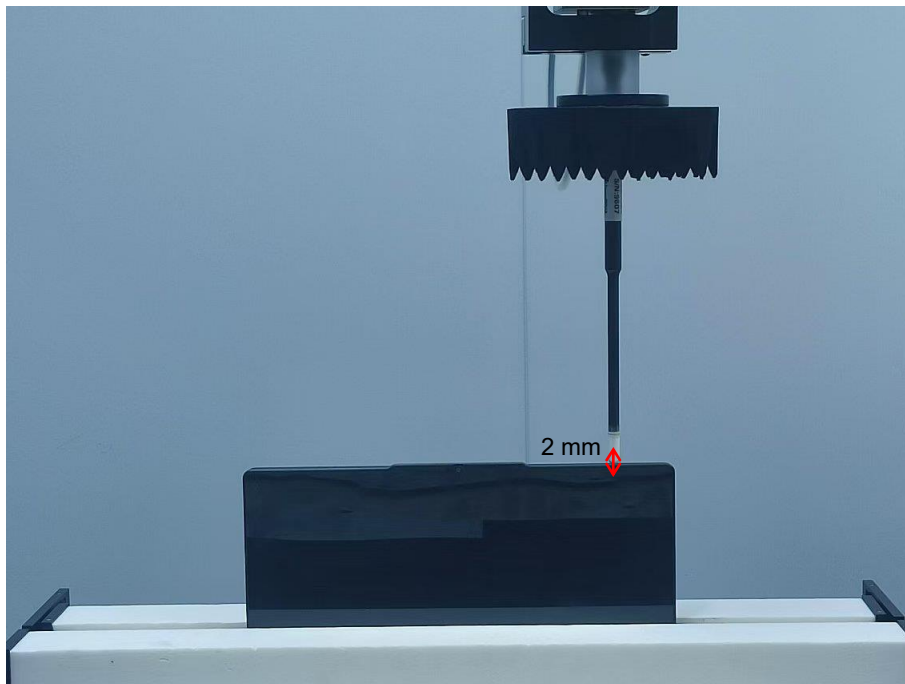
Top Edge (Tablet) (2mm)
