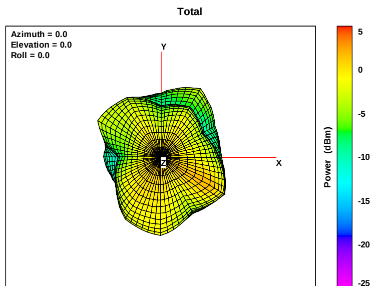
Max Antenna 3D Radiation Pattern 6525-6875 MHz
