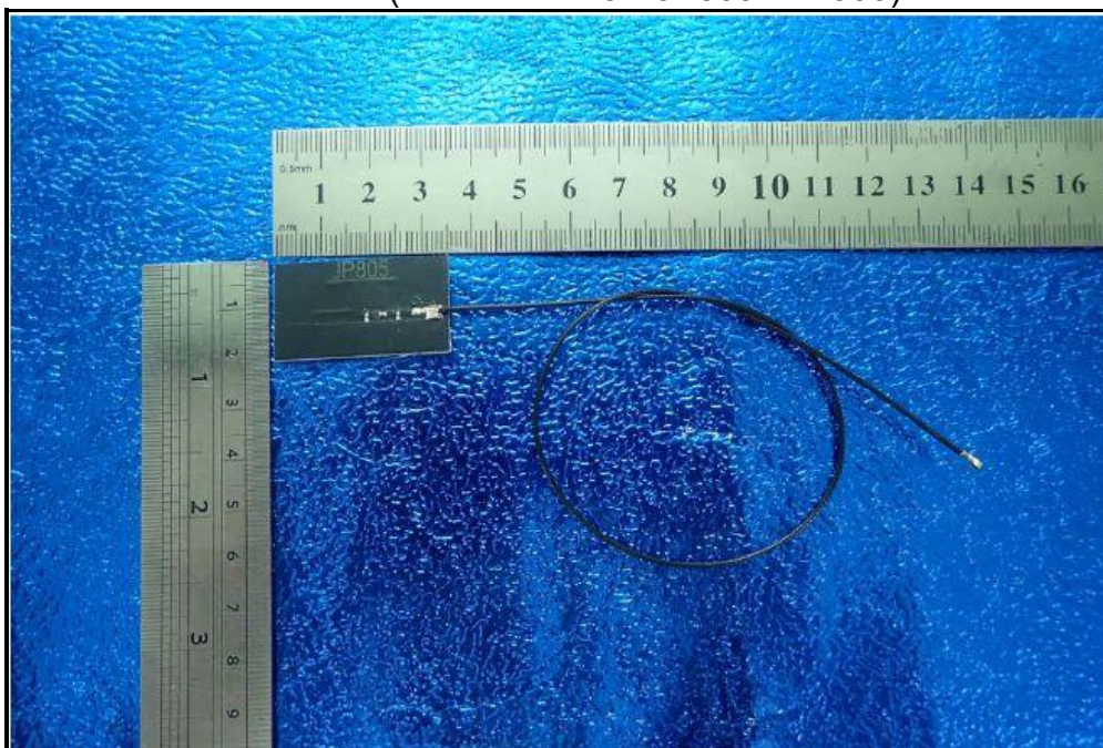
Antenna 2 (Model: RFA-57-JP805-4B-300)
