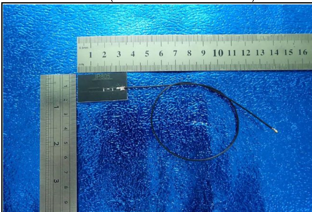
ANT Set 2 (Model: RFA-57-JP805-4B-300)
