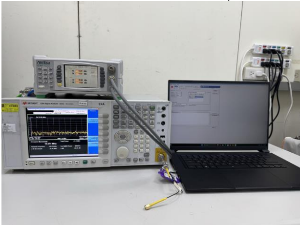
FCC_15_247_BLE_Conducted_Setup
