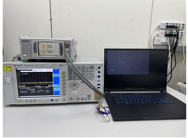
FCC_15_407_Conducted_Setup
