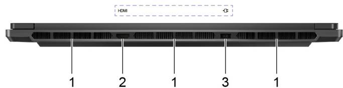
Figure 5. Legion Slim 7 16IRX9—rear-side view
