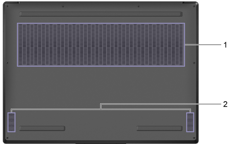
Figure 6. Legion Slim 7 16IRX9—bottom view
