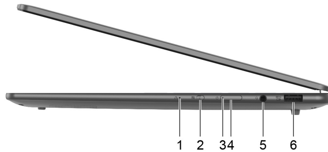
Figure 4. Yoga Slim 7 14IMH9—right—side view
