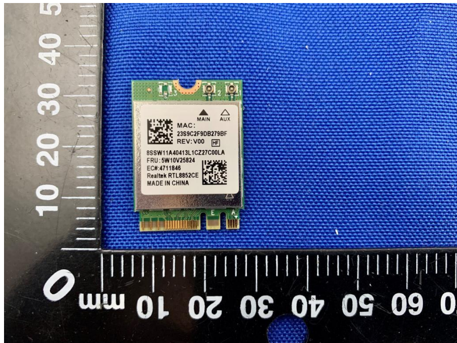
RF MODULE TOP VIEW-RTL8852CE (WITH SHIELDING)
