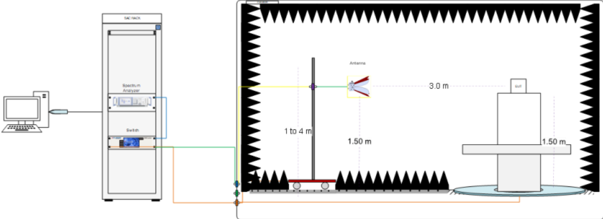
Radiated Setup 1 GHz – 6.4 GHz
