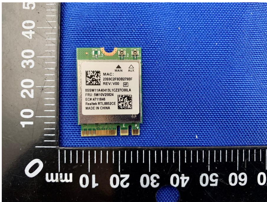
RF MODULE TOP VIEW-RTL8852CE
