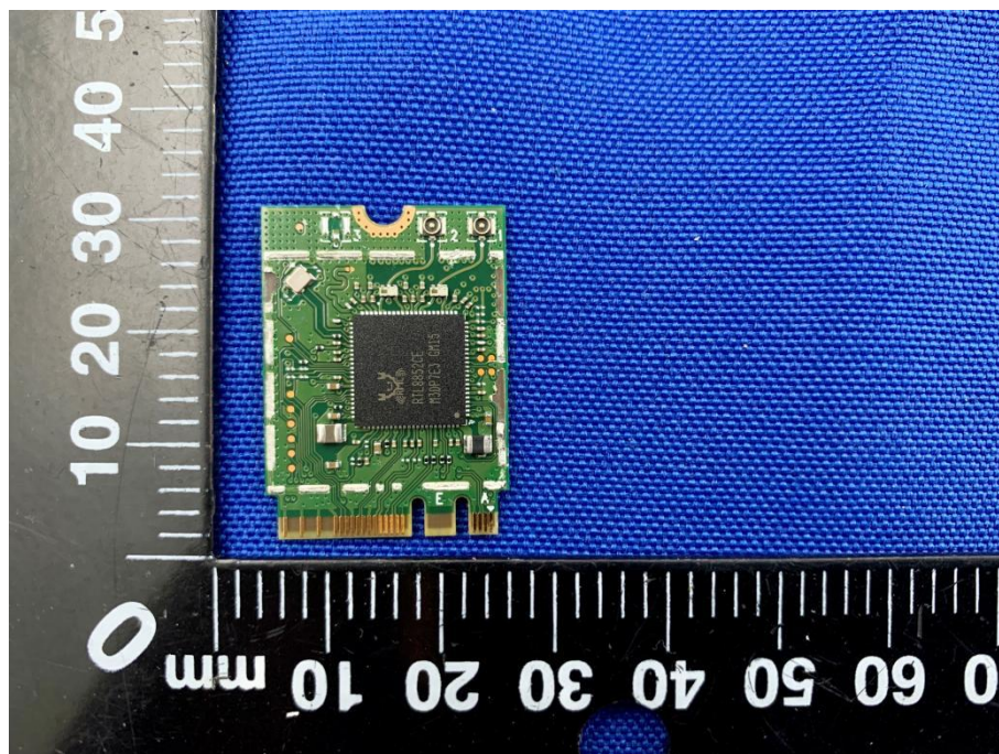
RF MODULE TOP VIE(WITHOUT THE SHIELDING)_RTL8852CE
