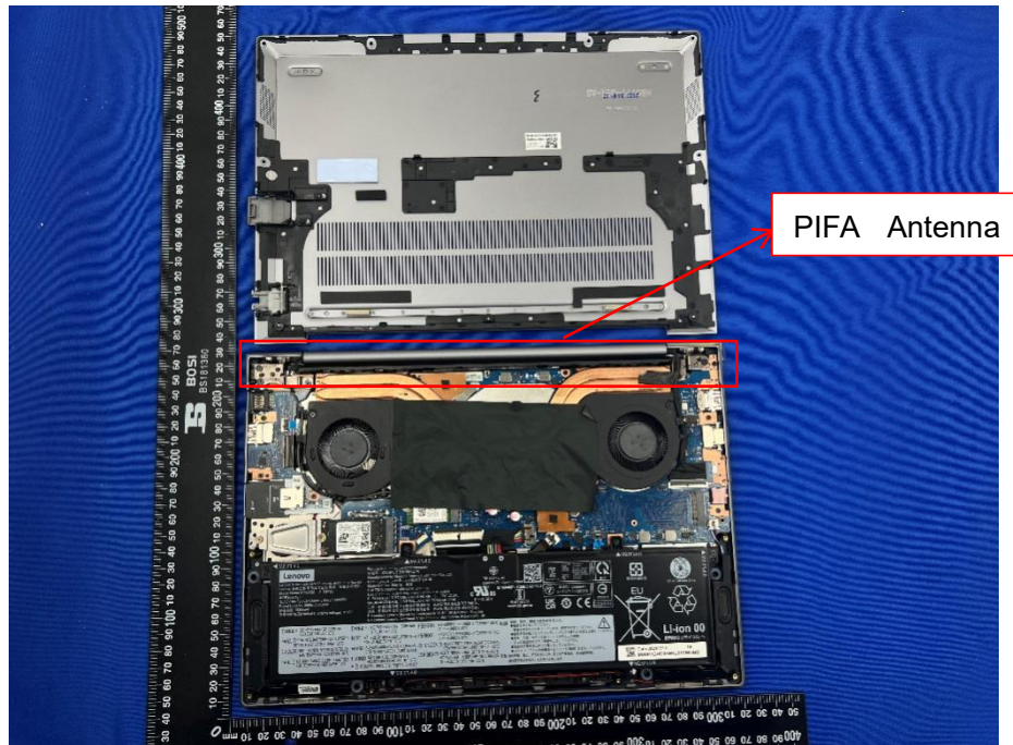
EUT UNCOVER VIEW 1
