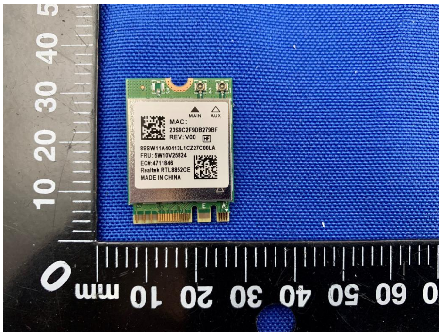
RF MODULE BACK VIEW_ RTL8852CE
